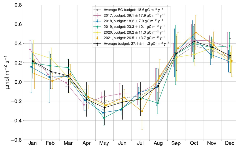
Figure 9. (a) Daily means of the seawater p_{CO_2} at the depth of 4.5 m at Utö in 2017–2021. Interpolated observations are shown with dotted line. (b) Monthly average CO_2 air-sea fluxes. The error estimates are explained in the Appendix.
