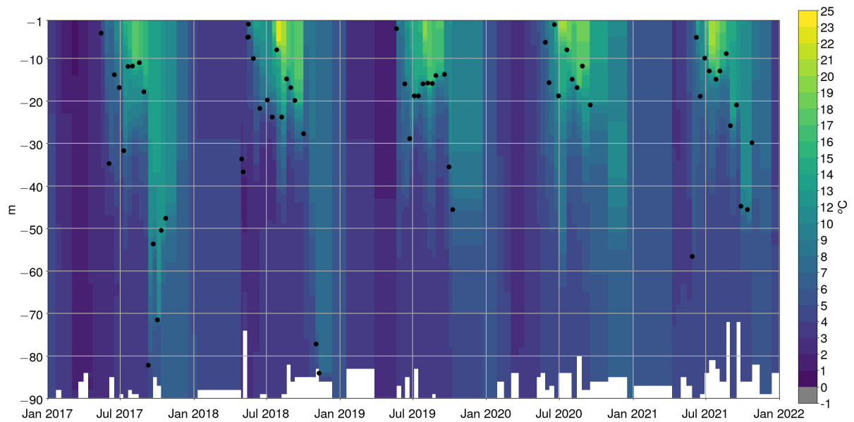
Figure 4. Temperature vertical profiles (colours) and the thermocline depths (dots) at Utö for the years 2017–2021, derived from the casts.
