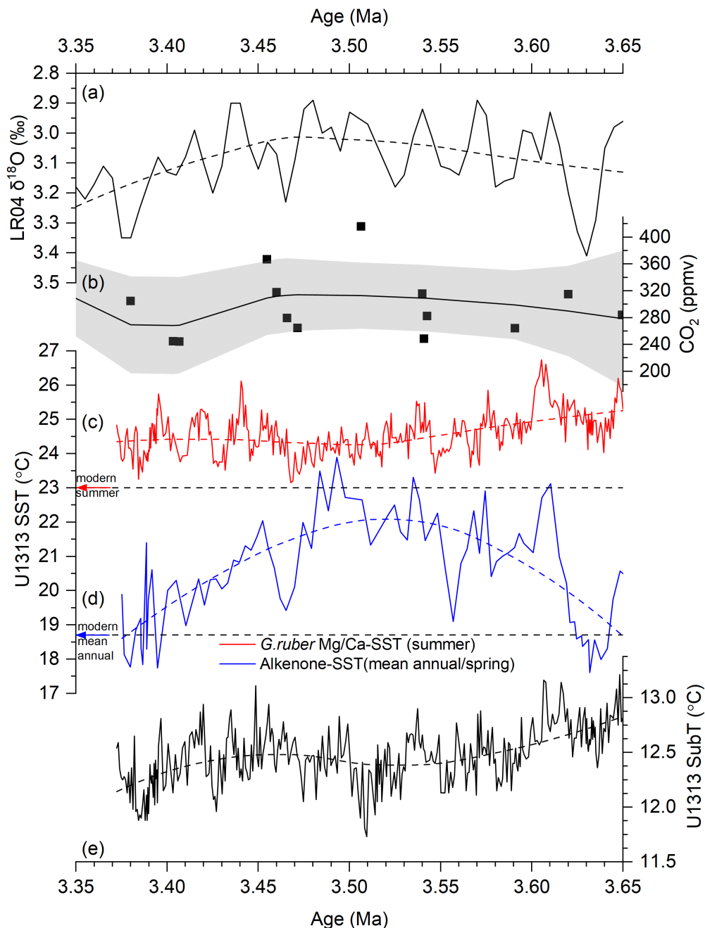
325 Figure 4. Distinct seasonal changes of SST records at Site U1313 during the early Late Pliocene. (a) The LR04 global benthic \delta^{18}\text{O} stack (Lisiecki and Raymo, 2005). (b) Paleo- \text{CO}_2 data available during the study interval (CenCO2PIP Consortium et al., 2023), with the black line indicating the smoothed curve with 95% confidence interval. (c) G. ruber white Mg/Ca-based summer SST. (d) Alkenone-based SST
