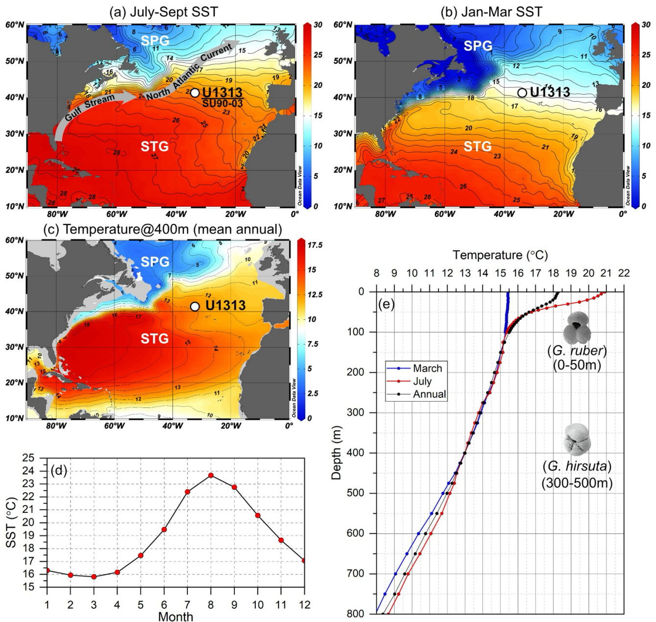
165 Figure 1. The location of Site U1313 and modern oceanographic settings. (a) Summer season (July to September) mean surface temperature. The main route of warm current Gulf Stream and its northern extension, the North Atlantic Current, are also presented. STG is subtropical gyre, SPG is subpolar gyre. Site SU90-03 (40.51°N; 32.05°W) which provides core top Mg/Ca ratios is presented by the same point of U1313 (41.00°N; 32.96°W) due to the proximity of locations. (b) Winter season (January to March) mean surface temperature and (c) mean annual water temperature at depth of 400 m. (d) Modern monthly mean surface temperature at site U1313, averaged from 2000–2015 derived from the Simple Ocean Data Assimilation (SODA) database (Carton and Giese, 2008). (e) Depth profile of temperature during different seasons 170
