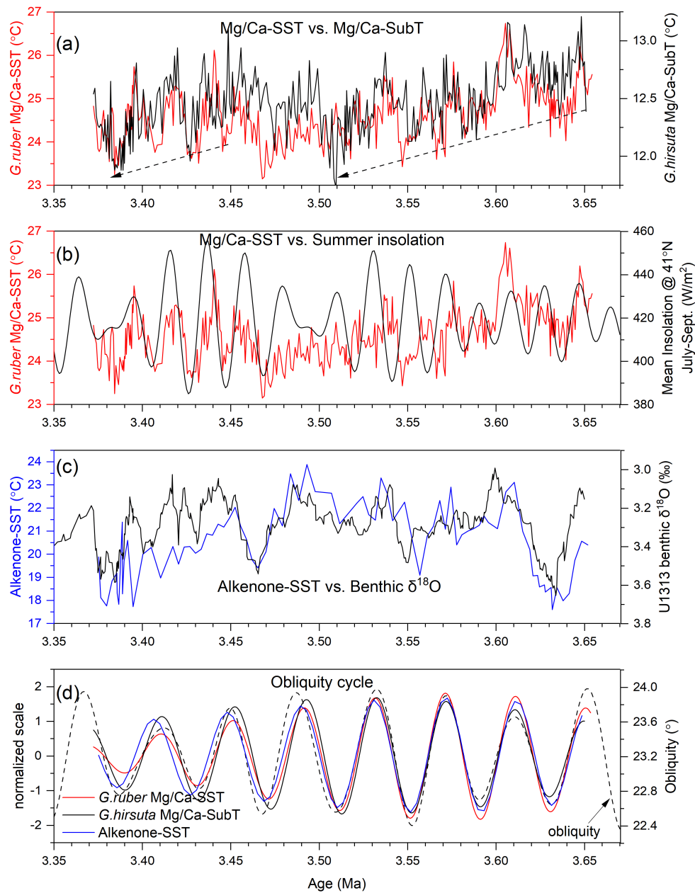
370 Figure 5. Comparison of G. ruber white Mg/Ca-based SST and G. hirsuta Mg/Ca-based SubT. (a) G. ruber white Mg/Ca-based SST (red) and G. hirsuta Mg/Ca-based SubT (black) records, with dashed arrows indicating long-term trends. (b) The comparison between G. ruber white Mg/Ca-based SST and mean insolation of July to September at 41°N (Laskar et al., 2004). (c) Comparison between the LR04 benthic \delta^{18}\text{O} stack (Lisiecki and Raymo, 2005) and the alkenone-based SST (Naafs et al., 2010). (d) Comparison between obliquity and filtered Mg/Ca-based SST, SubT and alkenone-based SST. Gaussian filtering, done with the software AnalySeries 2.0 (Paillard et al., 1996), centered at the frequency of 0.025 \pm 0.003 , i.e., the obliquity band.
