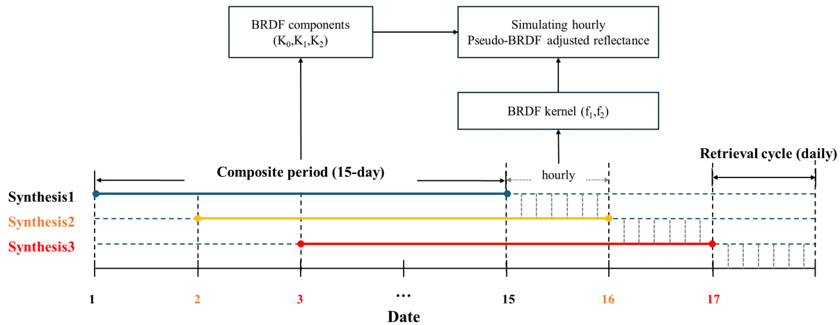
Figure 2. Schematic of 15-day composite period and retrieval cycle for BRDF modeling (The figure above has been updated to a revised version)
