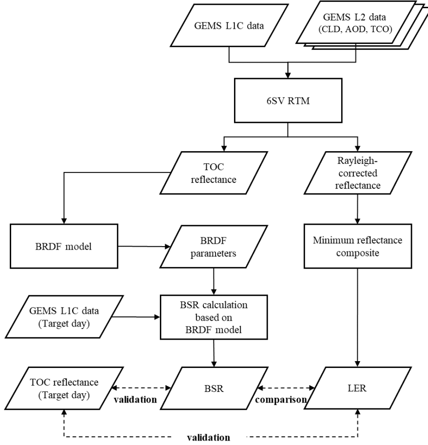
Figure 1. Flowchart of GEMS BSR algorithm Flowchart of this study
