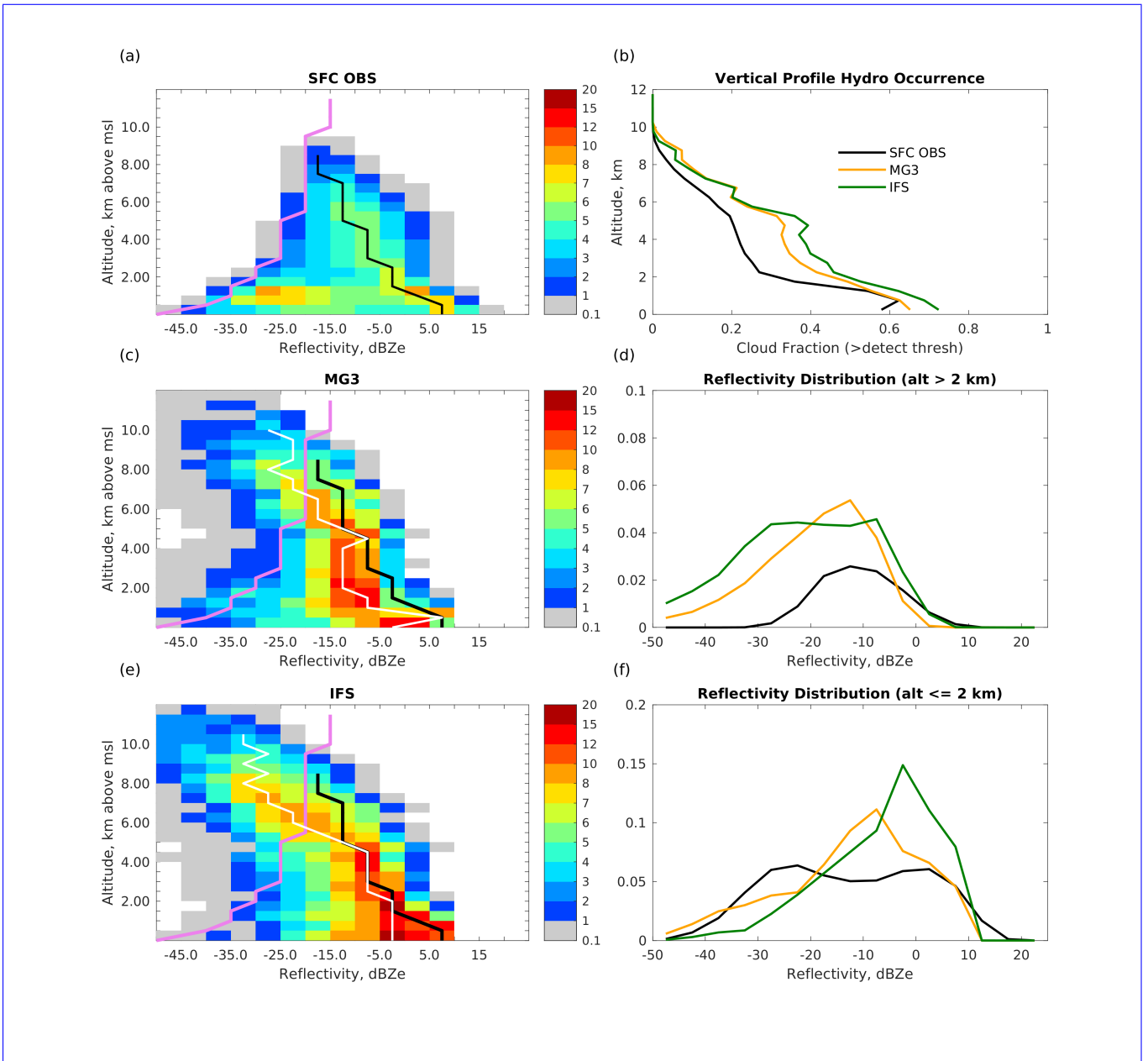
Figure 5. Left panels: Radar reflectivity-height histograms from (a) surface (vertically pointing W-band) radar, and from simulations using a radar-simulator with the (c) MG3 and (e) IFS microphysics. Colors indicate the fraction of time that hydrometeors are detected at the specified altitude and reflectivity. Histogram bins are 0.5 km x 5 dBZe. Violet line shows the Minimum Detectable Signal (MDS) of the surface radar. Black and white lines show the characteristic curve (see text) for observations (black, same in all panels) and simulations (white). Top-right: (b) profile of total hydrometeor occurrence, including only detections above the MDS (violet line). Middle-right: (d) Mean distribution of radar reflectivity for hydrometeors above 2 km altitudes (note occurrence in OBS is strongly affected by MDS below about -20 dBZe). Bottom-right: (f) Same as above (d) but includes only hydrometeors below 2 km (occurrence in OBS is unaffected by MDS above about -35 dBZe)
