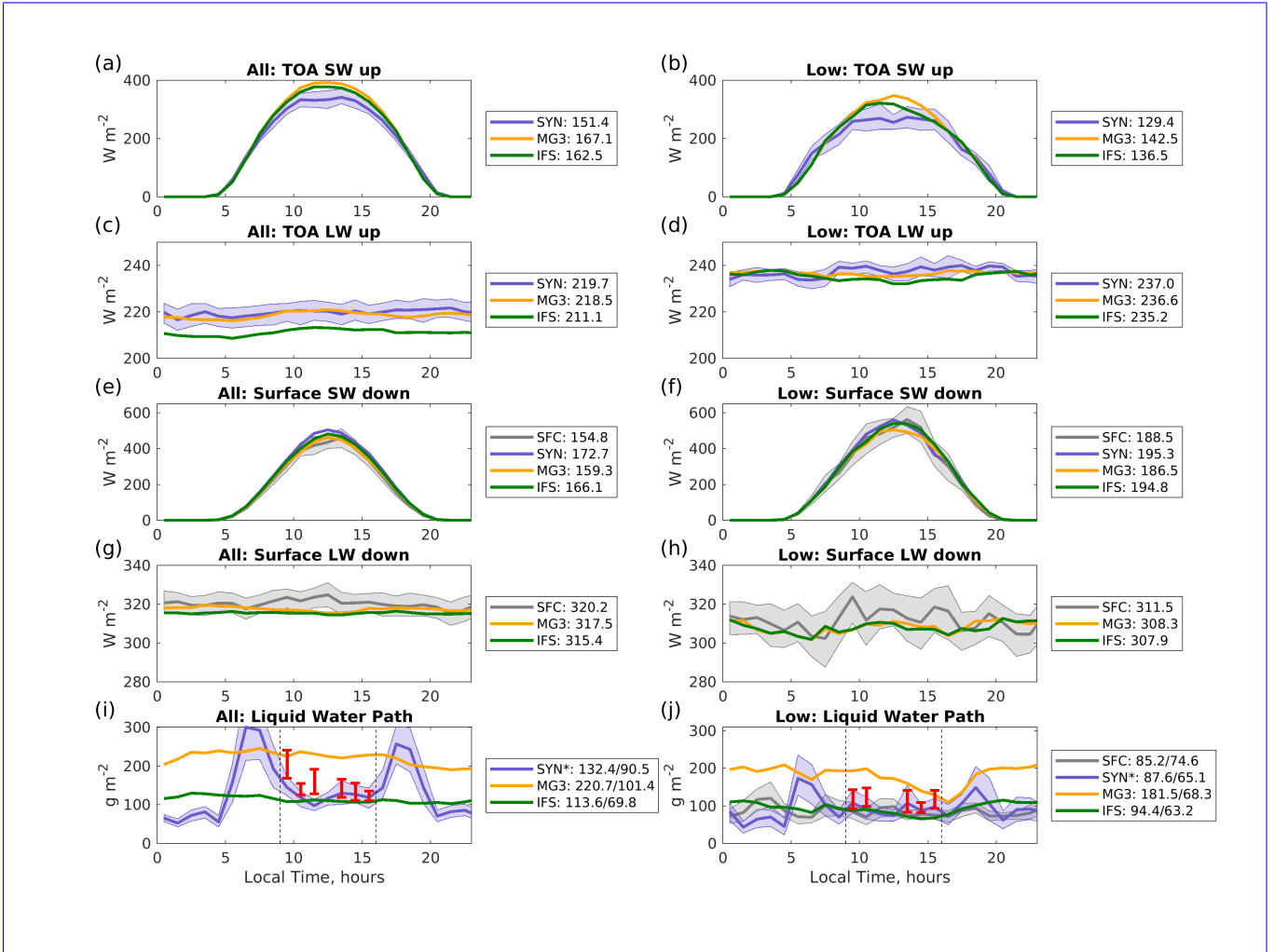
Figure 2. Mean diurnal cycles. Panels from top to bottom show the outgoing Outgoing TOA (a,b) SW and (c,d) LW flux, downward Downward surface (e,f) SW and (g,h) LW flux, and LWP. Left column (a,c,e,g,i) shows diurnal averages for all times and the right column (b,d,f,h,j) for periods when only low cloud (hydrometeors < 2 km) are present base don hourly average (simulated or observed) radar reflectivity . In each panel, shading that surrounds the surface or satellite values depicts the estimated one-sigma sampling uncertainty for a particular hour over all days. Sampling uncertainty for all datasets is of similar magnitude. The bottom panel in each column shows the diurnal cycle of LWP is also shown for all times (i) and just low cloud periods (j) . CERES SYN retrieved LWP in purple (which combines geostationary and MODIS data). MODIS only (red symbols) as described in the text. The legend gives the daily mean for each dataset, and for LWP both the daily mean and median are given. CERES SYN means and medians are restricted to data collected between 9 and 16 hours local time (see text).
