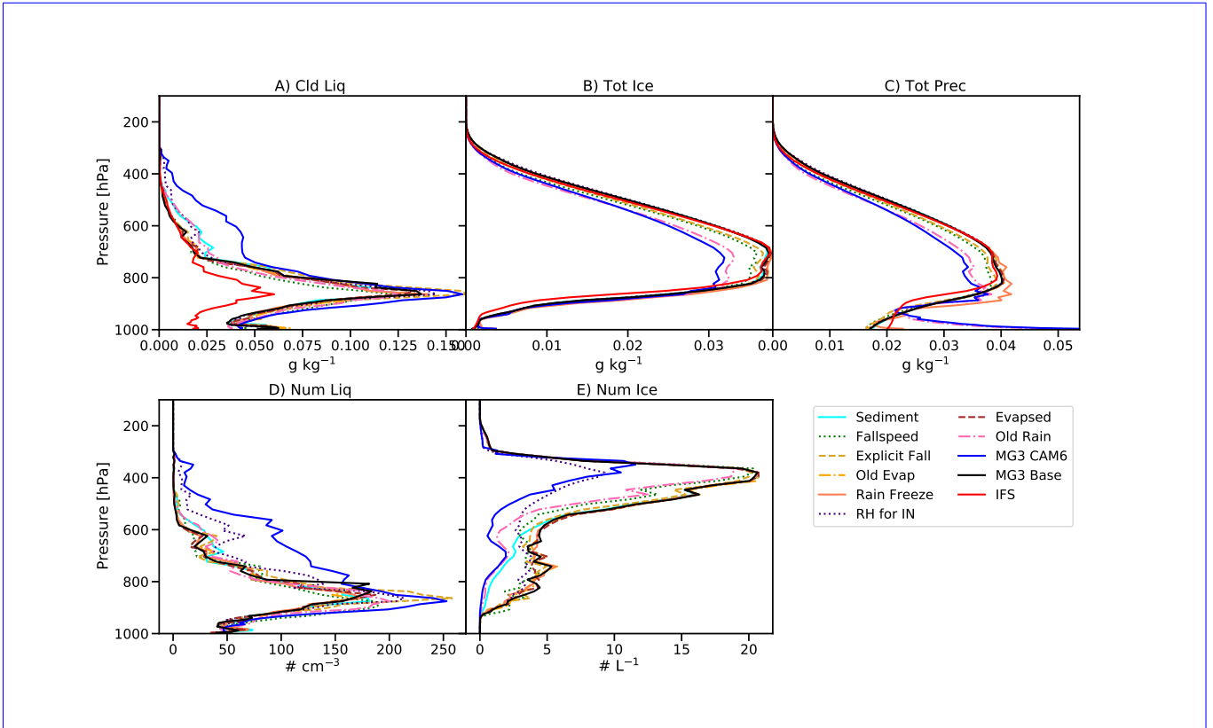
Figure 9. Vertical time averages of A) Supercooled liquid water, B) Total ice (ice+snow+graupel), C) Total precipitation, D) Liquid number concentration, E) Ice number concentration, for the MG3 base version (black solid) and various MG3 microphysics sensitivity tests as noted in the legend to differentiate MG3 and IFS microphysics. The reference IFS microphysics is included in A,B,C (red solid).
