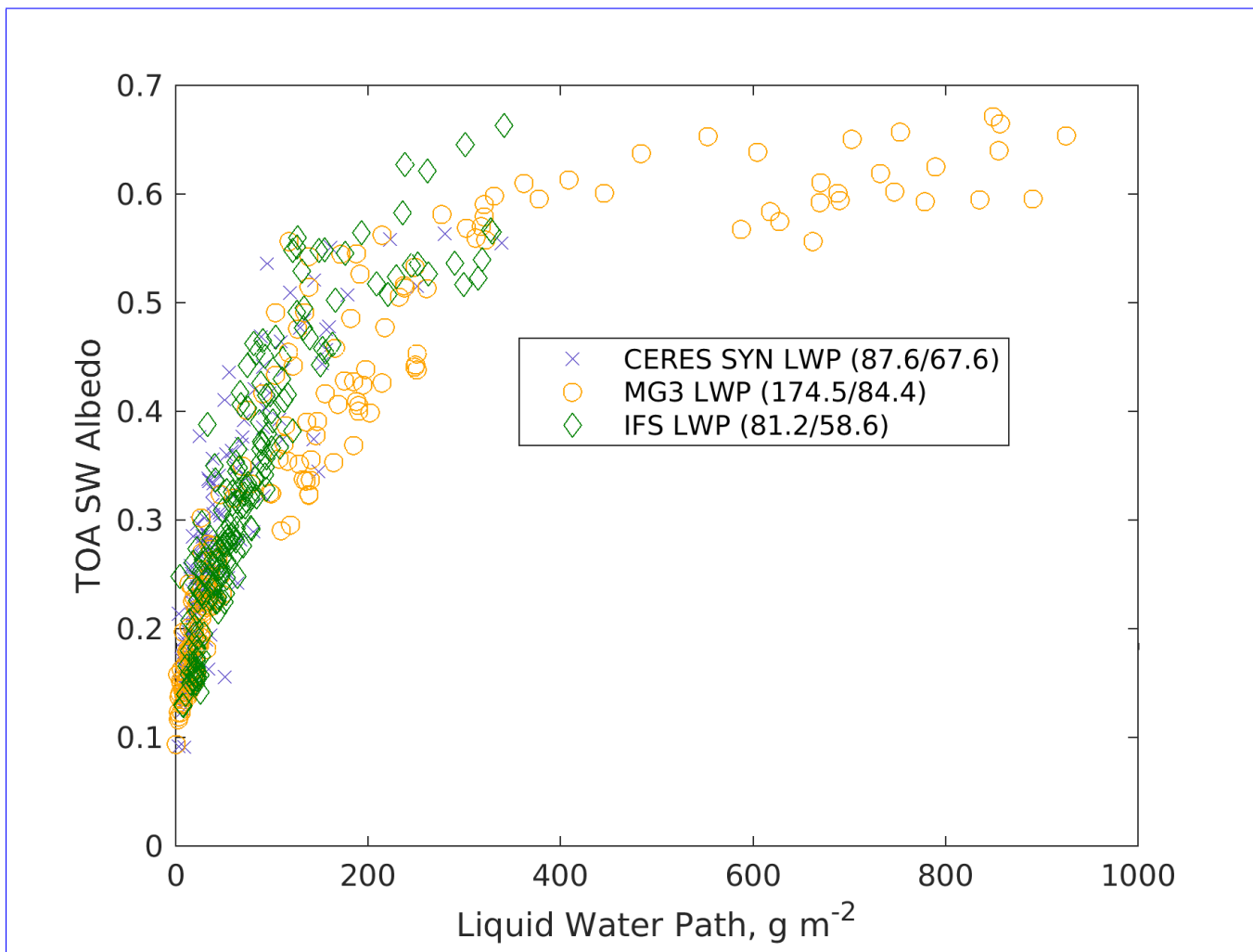
Figure 3. TOA SW albedo from CERES SYN as a function of in-cloud liquid water path (LWP) for low-cloud periods during daylight (local time from 9 to 16 hours) from CERES Observations (purple cross), MG3 simulation (orange circles) and IFS simulation (green diamond). Legend shows the mean/median LWP.
