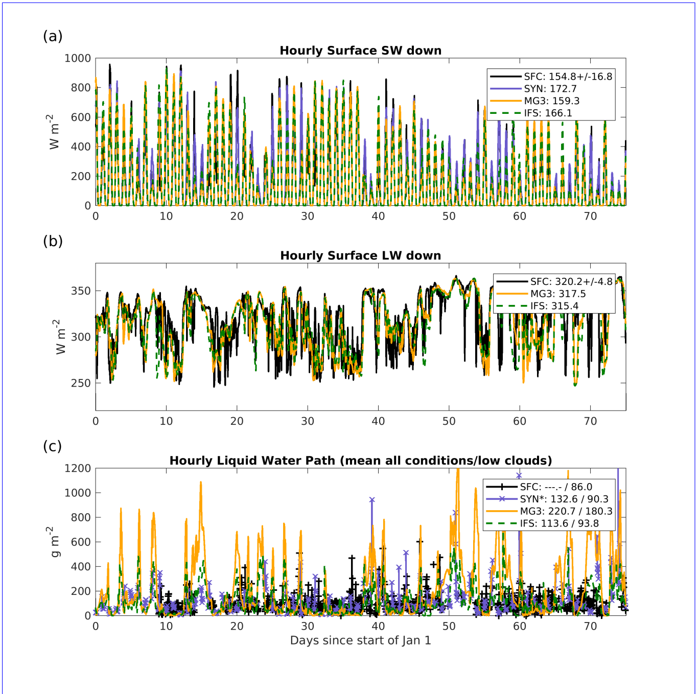
Figure 1. Time series of hourly averaged values: ( top-panel ) downward surface shortwave (SW) flux, ( middle-panel ) downward longwave (LW) flux, and ( bottom-panel ) liquid water path (LWP). For each dataset the legend gives the mean value, and for the SW and LW flux, the estimated one-sigma uncertainty in the mean is also given. For LWP, the legend gives the mean value for all times followed by the mean restricted to periods where only low clouds are present (see text). Surface observations (Black Solid and tick) , MG3 microphysics (Orange Solid) , IFS microphysics (Green Dashed) . The CERES SYN data ( Purple Solid and cross ) and average values are also restricted to data collected between 9 and 16 hours local time to avoid biases associated with low solar zenith angles (see text).
