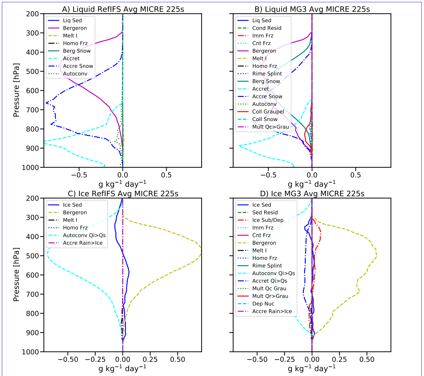
Figure 7. Profiles of (A,B) cloud liquid water and (C,D) cloud ice process rates, A,C) for the IFS microphysics and B,D) for MG3. Process rates are described in Table A1.
