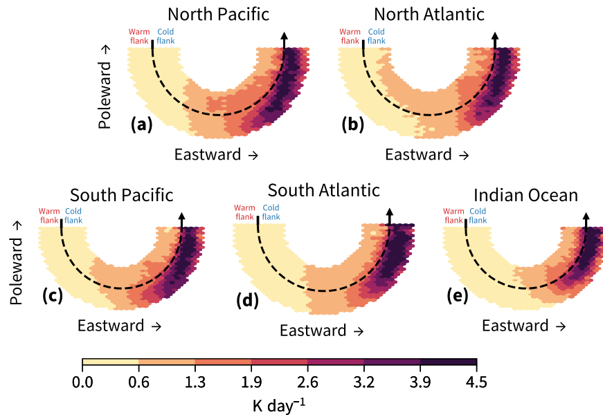
Figure 9. Like Fig. 7c for 3h-2D jets, showing latent heating for the five major storm track regions (Fig. 8f) in their respective winter season. The axis direction "poleward" is northward in the NH and southward in the Southern Hemisphere.
