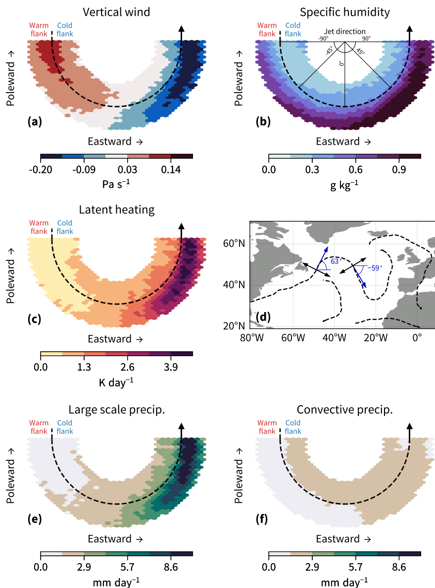
Figure 7. Cross sections for vertical wind (a; 700–200hPa); specific humidity (b; 700–200hPa); latent heating (c; 700–200hPa); large-scale precipitation (e); and precipitation from the convection scheme in ERA5 (f) for the 3h-2D jets. The cross sections are sorted by the jet direction and shown with their original orientation in the longitude–latitude plane. The jet directions are parallel to the orientation of the jet core (black dashed line). The angles given in (b) refer to the jet direction. Jet directions with < 0^\circ have a poleward component, with = 0^\circ are perfectly zonal, and with > 0^\circ have an equatorward component. Jet directions of two illustrative cross sections are shown in blue in panel (d). Only jet directions between -90^\circ and 90^\circ are shown. The data are spatially binned and averaged using 30 bins in both the horizontal and vertical direction.
