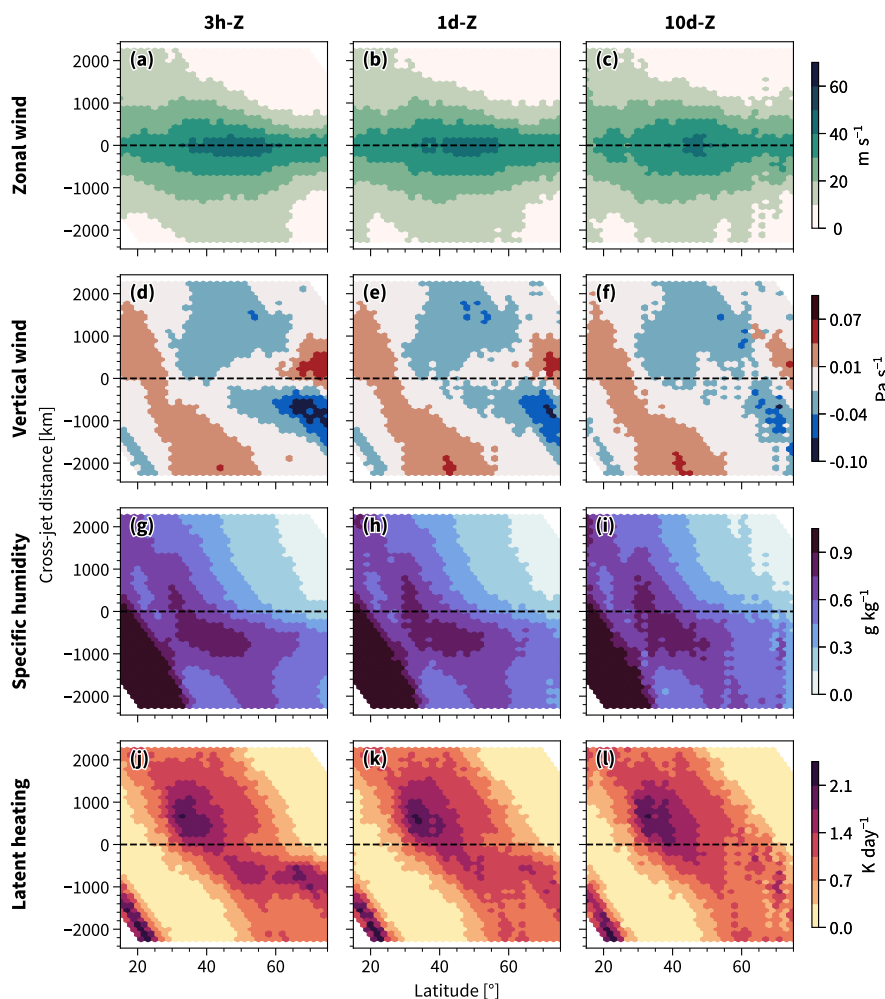
Figure 3. Three-hourly zonal wind (2 PVU; a–c), vertical wind (700–200 hPa; d–f), specific humidity (700–200 hPa; g–i) and latent heating (700–200 hPa; j–l) averaged from 60° W to 0° E and shown against the latitude of the concurrent 3h-Z jet (left), 1d-Z jet (middle), and 10d-Z jet (right). The jet core is shown by the black dashed line. The data are spatially binned and averaged over, using 30 bins in the horizontal and 20 bins in the vertical direction.
