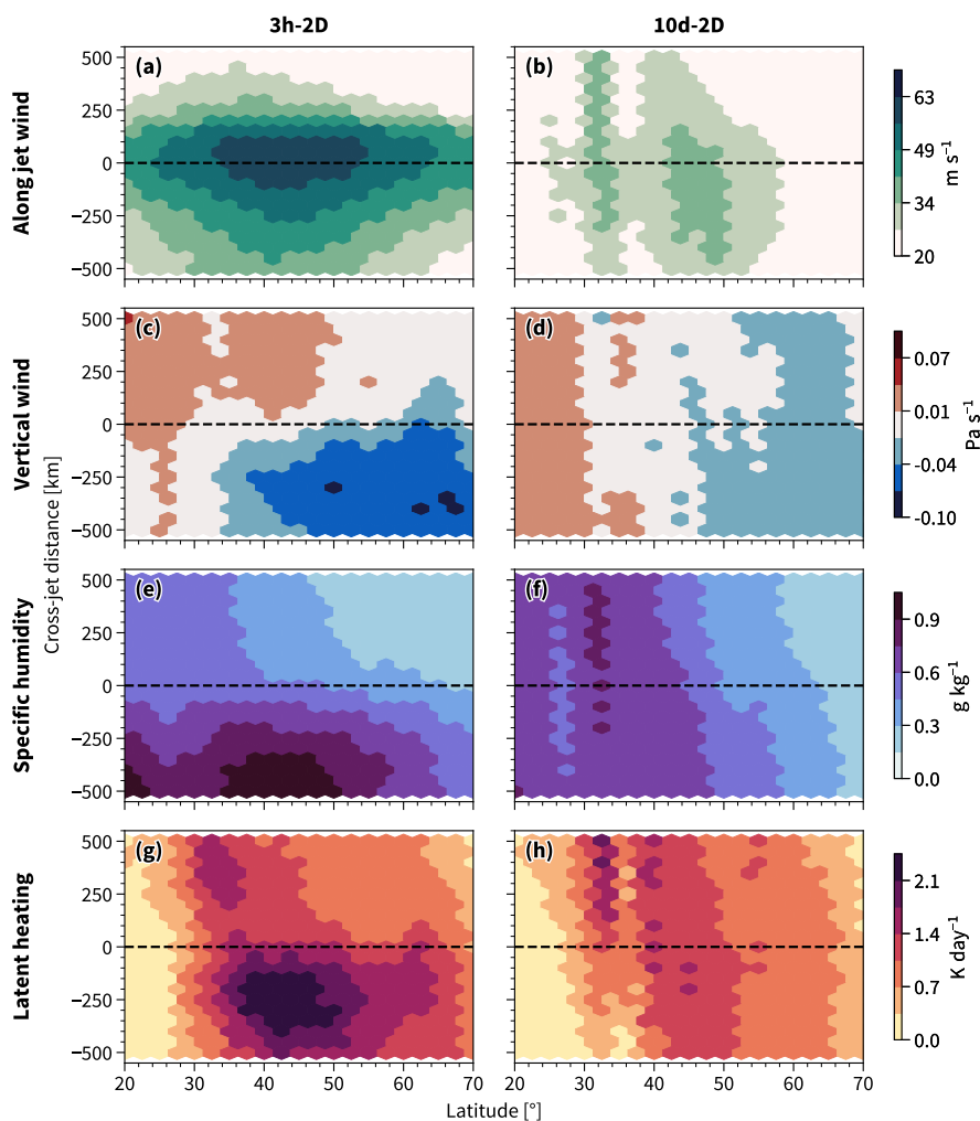
Figure 5. Three-hourly winds in the direction of the jet (2 PVU; a–b); vertical wind (700–200 hPa; c–d), specific humidity (700–200 hPa; e–f) and latent heating (700–200 hPa; g–h) interpolated to the cross sections sampled from the two-dimensional jets: 3h-2D (left) and 10d-2D (right). Data are plotted against the latitude of the jet core of each cross section. The warm flanks of the jets lie below- and the cold flanks above the black dashed line, which denotes the jet core. The data are spatially binned and averaged over, using 20 bins in the horizontal and 10 bins in the vertical direction.
