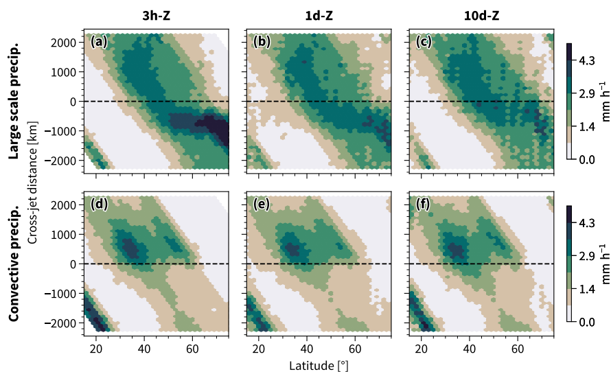
Figure 4. Like Fig. 3 but for large-scale precipitation (a–c) and precipitation from the ERA5 convection scheme (d–f).
