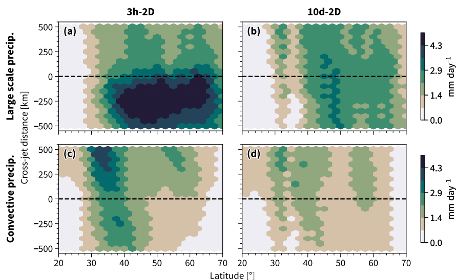
Figure 6. Like Fig. 5 but for large-scale precipitation (a–b) and precipitation from the ERA5 convection scheme (c–d) conditional on the 3h-2D jet axes (left) and the 10d-2D jet axes (right).
