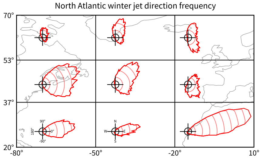
Figure B1. Wind roses that comprise the jet directions of the 100,000 cross sections sampled in the North Atlantic winter. The grid shows the sampling region for each wind rose. The black circles correspond to 50 cross sections and the red contours: 100, 200, 300, 400, 500, 600, 700, and 800 cross sections.
