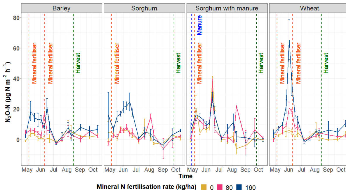
290 Figure 5: N 2 O emissions ( \mu\text{g N m}^{-2} \text{h}^{-1} ) according to crop types and fertilisation rates during the study period.
