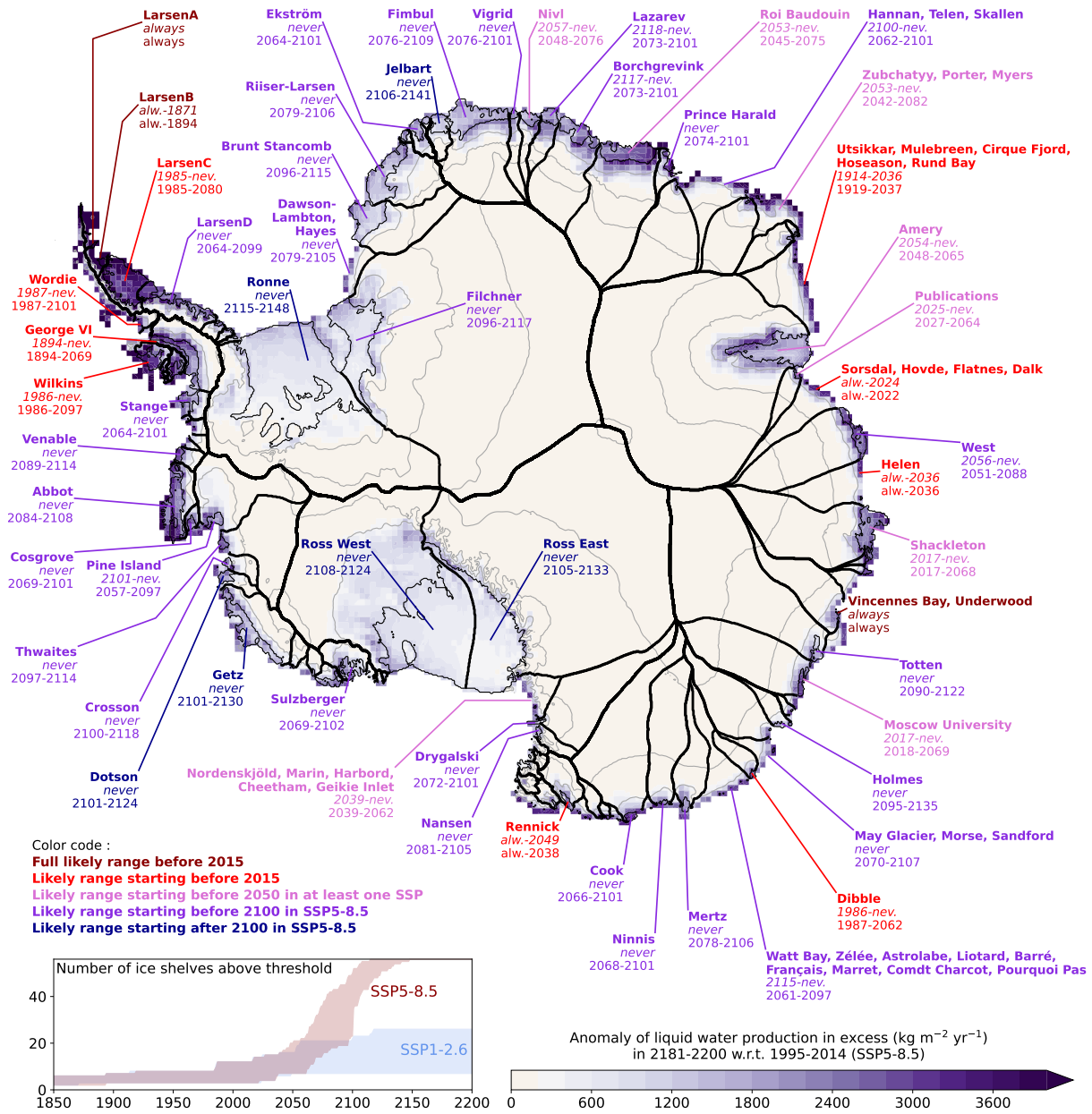
Figure 12. Time intervals at which the likely (17–83 th percentiles) production of excess liquid water likely exceeds the threshold that makes hydrofracturing possible (see text), for 56 ice shelves or groups of ice shelves. The first time range, in italic , corresponds to SSP1-2.6, while the second range corresponds to SSP5-8.5. The estimated years are based on the weighted 16-model ensemble until 2100 and on the weighted 8-model ensemble from 2101 to 2200. Indications of "always" and "never" have to be understood as between 1850 and 2200 (e.g., "never" means either after 2200 or never). The background map shows the eight-model mean anomaly of liquid water production beyond firm saturation at the end of the 22 nd century. The topography contours are in grey (every 1000 m) and the ice shelves are delineated in thin black. The contours of the drainage basins of individual ice shelves is in thick black (from Mouginot et al., 2017 and Rignot et al., 2019).
