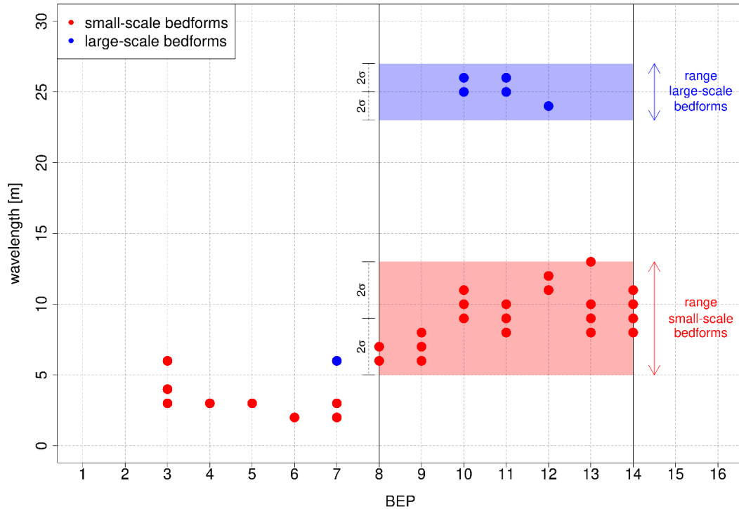
370 Figure 7: Derivation of the ranges of window sizes for the zerocrossing procedure from the identified predominant wavelengths in individual BEPs by means of wavelet analysis.
