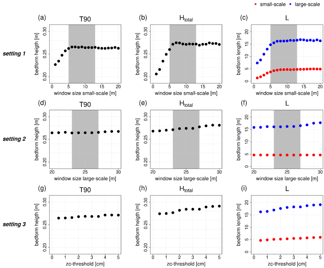
Figure 14: Influence of variation in the input parameters on derived bedform geometries (grey area corresponds to the selected value range based on the wavelet analysis). Setting 1: window size small-scale 1 m - 20 m, window size large-scale 25 m, zc-threshold 0.5 cm. Setting 2: window size small-scale 8 m, window size large-scale 20 m – 30 m, zc-threshold 0.5 cm. Setting 3: window size small-scale 8 m, window size large-scale 25 m, zc-threshold 0.5 cm – 5 cm.
