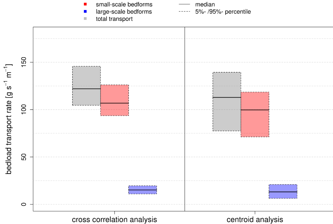
475 Figure 12: Comparison of bedload transport rates derived from cross-correlation and centroid analysis along the evaluated BEP.
