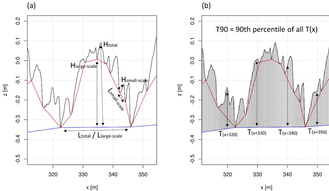
225 Figure 3: (a) – Definition of individual bedform attributes. (b) – Determination of the T90-parameter.
