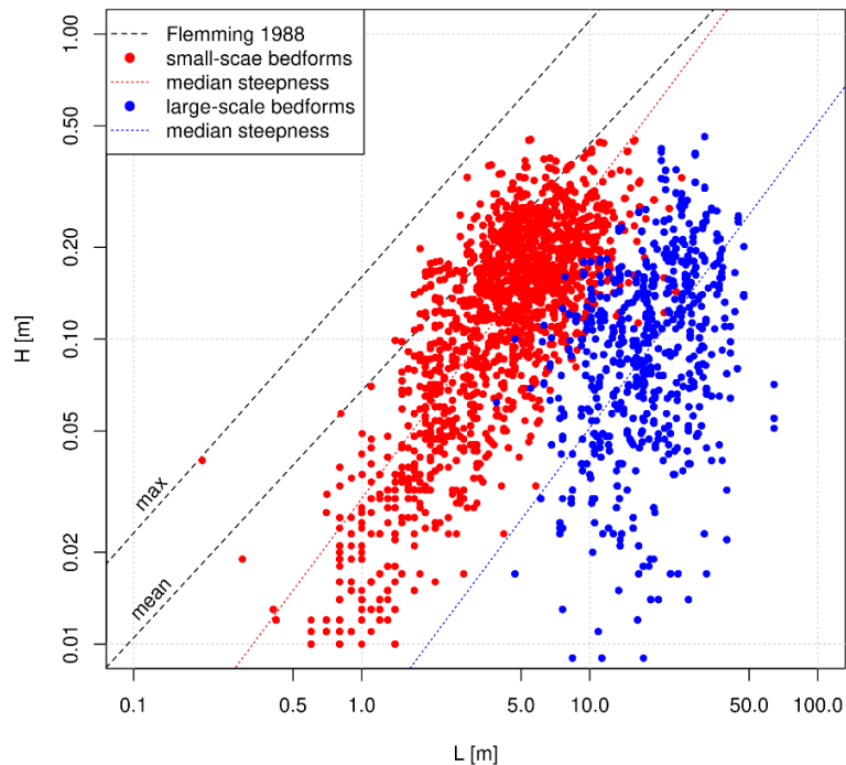
515 Figure 13: Ratio of identified bedform heights and lengths obtained from MBES-data from Lower Rhine (February 2020) compared to mean and maximum bedform height according to Flemming (1988).
