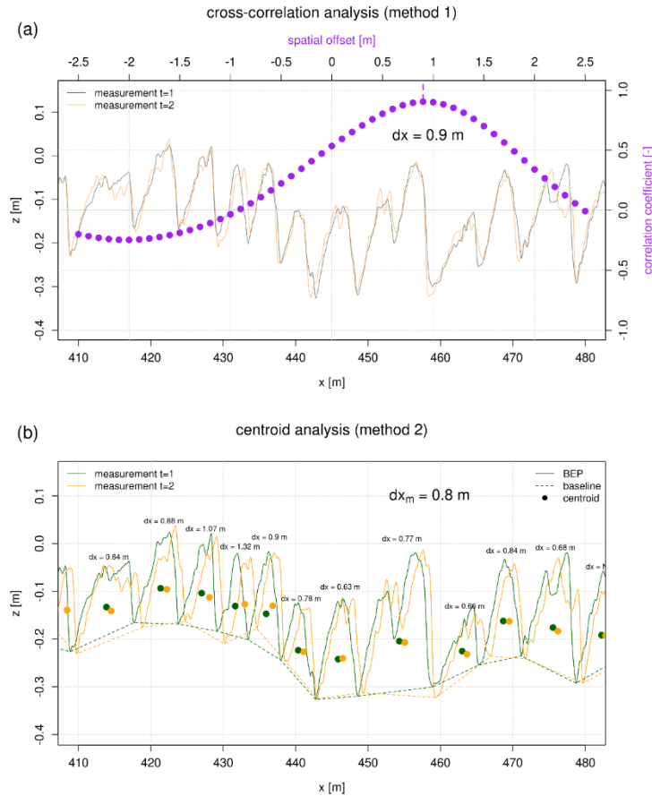
Figure 4: Calculation of bedform migration based on the cross-correlation analysis (a) and by comparing the geometrical centroids individual bedform areas (b). The time difference between both measurements was 0.4 h (corresponding to measurement pair no. 2 in Table A3, Appendix A).
