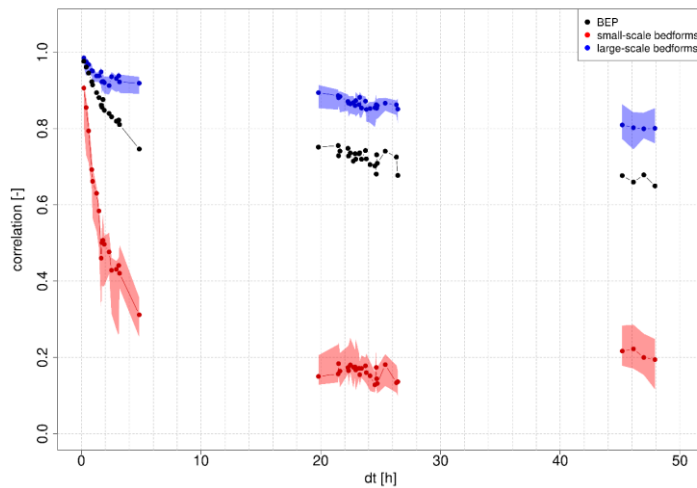
Figure 9: Correlations coefficients from the cross-correlation analysis (method 1) as a function of time difference between successive measurements. The red and blue dots represent the median values for small-scale and large-scale bedforms obtained from MCS. Polygons show the total range of results. For the total BEP only one results per measurement is available.
