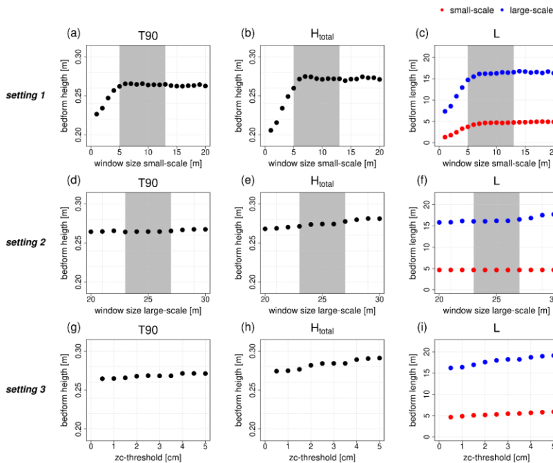
645 Figure 14 : Influence of variation in the input parameters on derived bedform geometries (grey area corresponds to the selected value range based on the wavelet analysis). Setting 1 : window size small-scale 1 m - 20 m, window size large-scale 25 m, zc-threshold 0.5 cm. Setting 2 : window size small-scale 8 m, window size large-scale 20 m – 30 m, zc-threshold 0.5 cm. Setting 3 : window size small-scale 8 m, window size large-scale 25 m, zc-threshold 0.5 cm – 5 cm.
