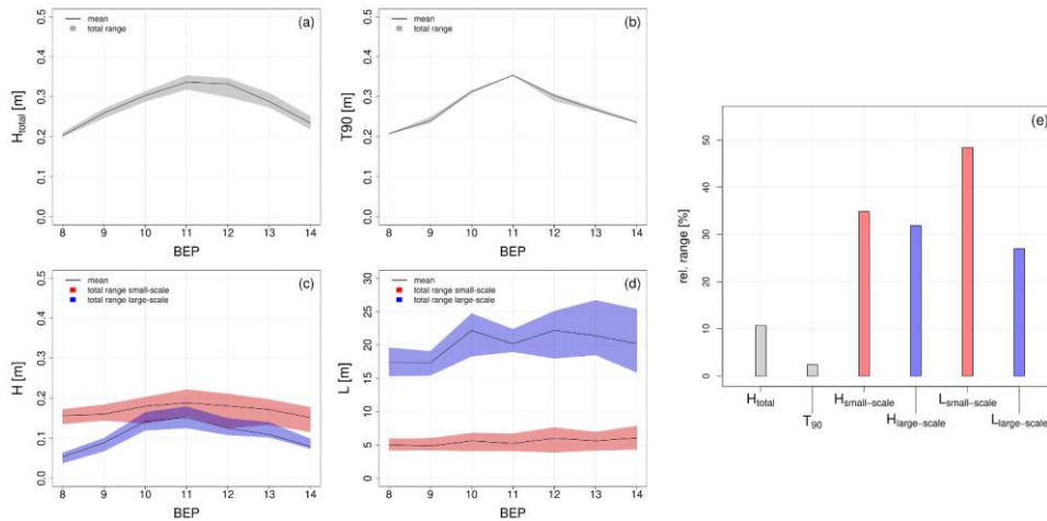
Figure 89: Resulting bedform parameters of the Monte Carlo Simulation. (a-d) - Identified ranges and mean values for individual BEPs. (e) - Averaged relative ranges over BEPs 8-14.
