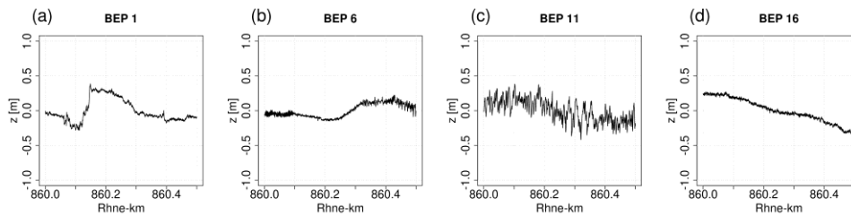
Figure 6: Selected BEPs derived from MBES-data of the first measurement from 17 February 2020.
