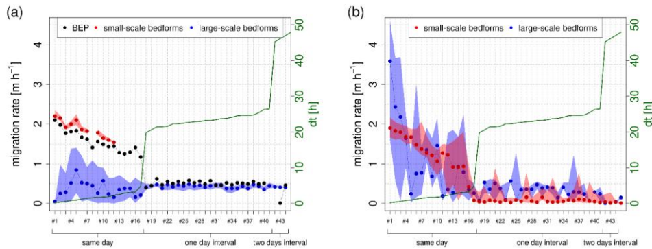
Figure 11: Calculated migration rates for all respected measurement pairs by means of cross-correlation analysis (method 1, a) and centroid analysis (method 2, b).
