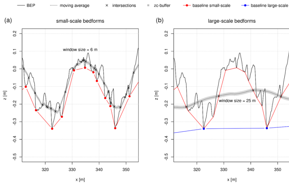
765 Figure A13: Zero-crossing procedure. (a) - Calculation of the baseline of the small-scale bedforms. (b) - Calculation of the baseline of the large-scale bedforms.
