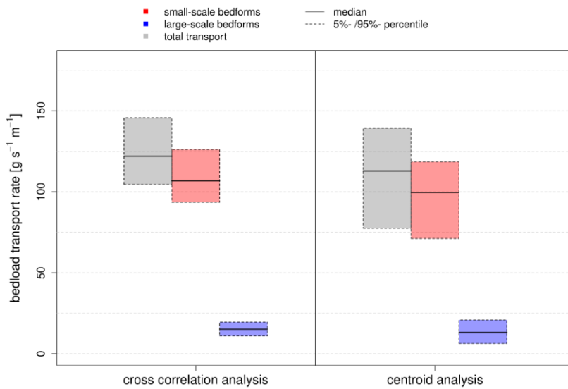
Figure 12.13: Comparison of bedload transport rates derived from cross-correlation and centroid analysis along the evaluated BEP.
