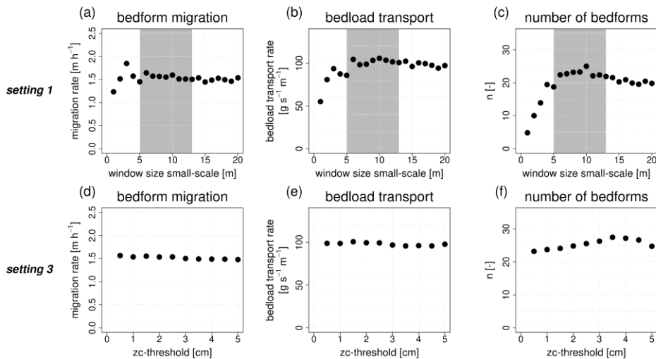
Figure 16: Influence of variation in the input parameters on the centroid analysis (grey area corresponds to the selected value range based on the wavelet analysis). Setting 1: window size small-scale 1 m - 20 m, window size large-scale 25 m, zc-threshold 0.5 cm. Setting 3: window size small-scale 8 m, window size large-scale 25 m, zc-threshold 0.5 cm - 5 cm.
