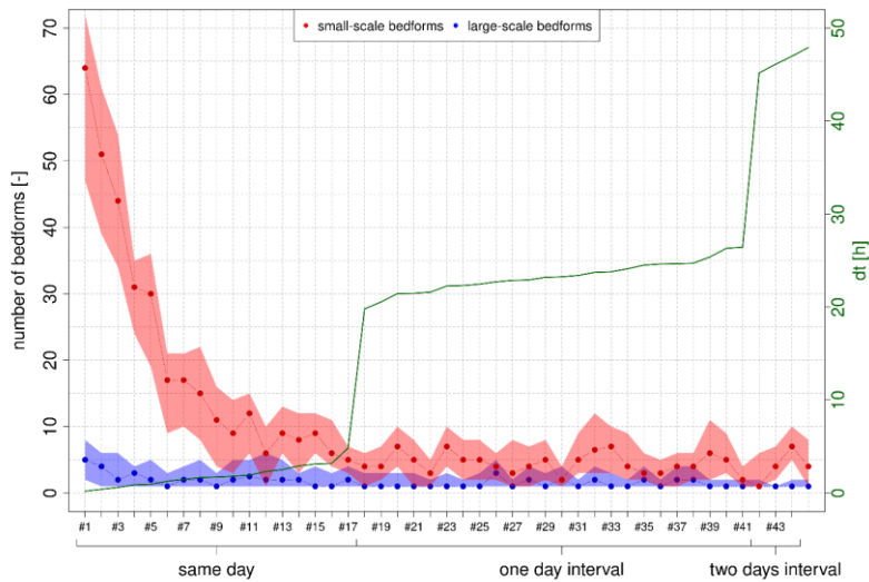
455 Figure 1014: Number of traceable bedforms depending on measurement interval (centroid analysis, method 2). The red and blue dots represent the median values for small-scale and large-scale bedforms obtained from MCS. Polygons show the total range of results.
