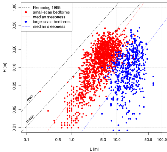
Figure 13-14: Ratio of identified bedform heights and lengths obtained from MBES-data from Lower Rhine (February 2020) compared to mean and maximum bedform height according to Flemming (1988).
