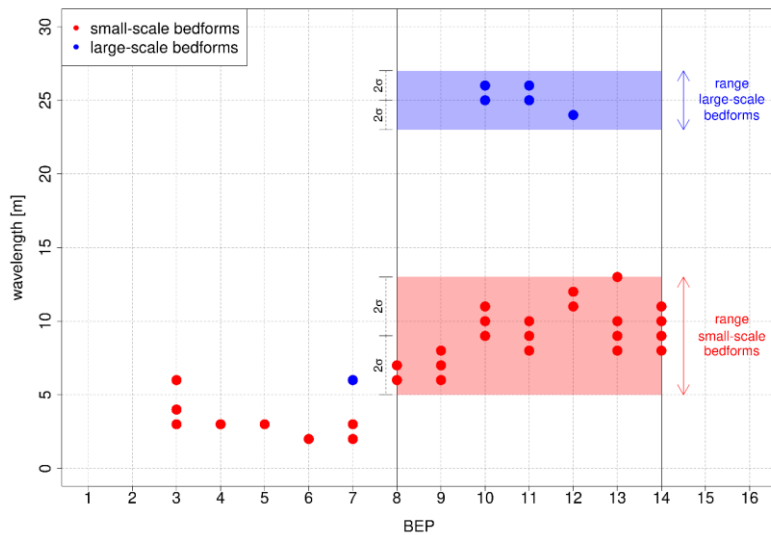
395 Figure 78: Derivation of the ranges of window sizes for the zerocrossing procedure from the identified predominant wavelengths in individual BEPs by means of wavelet analysis.
