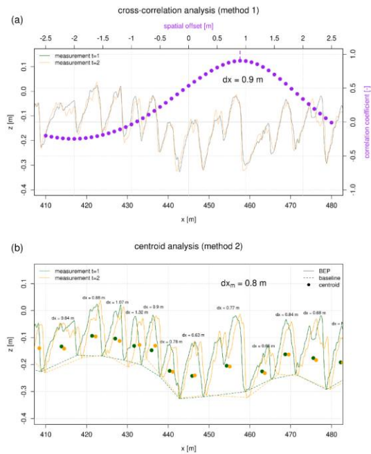
Figure 45: Calculation of bedform migration based on the cross-correlation analysis (a) and by comparing the geometrical centroids individual bedform areas (b). The time difference between both measurements was 0.4 h ( corresponding to measurement pair no. 2 in Table A3, Appendix A ).
