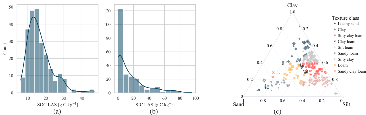
Figure 1. Distributions of SOC (a), SIC (b), and particle-size as a proportion of sand, silt, and clay (c), in the dataset of 240 samples, as measured by the LAS Saint-Laurent Blangy. SIC range is 0.5 to 96.8 g C kg -1 , and SOC range is 5.37 to 44.64 g C kg -1 .
