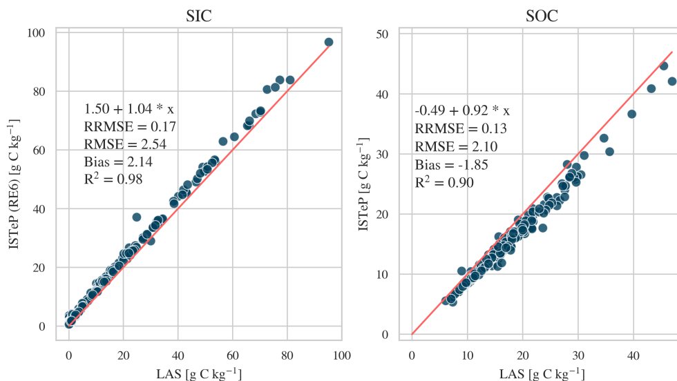
Figure 2. Comparison of the SIC and SOC measurements before correction from the RE6 analysis by ISTeP and reference measurements by LAS Saint-Laurent Blangy. The red line represents the 1:1 diagonal.
