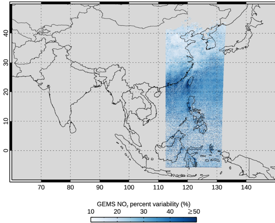
Figure A2: January 2023 monthly average of the GEMS NO 2 TrC relative daily variation (RDI) with respect to the 13:45 local time observed value at each location. Regions west of about 113° E and east of about 132° E are not mapped due to lacking observations at 13:45 local time.
