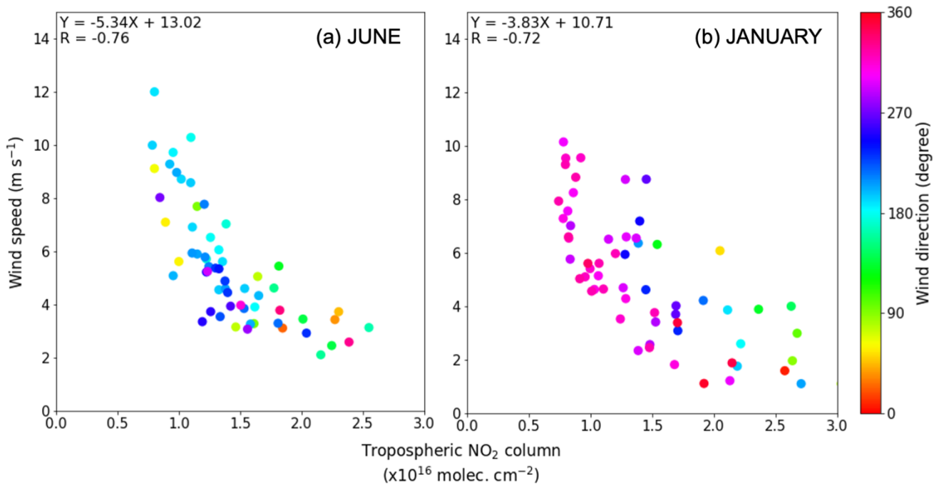
430 Figure 12: Scatterplot of the MUSICA v0 average daily NO 2 TrC compared to the magnitude and direction of the prevailing model surface layer wind (usually around ~120 m) over Seoul for June and January combined data for in the two years 2022 and 2023. Constant anthropogenic emissions during the day (Base case).
