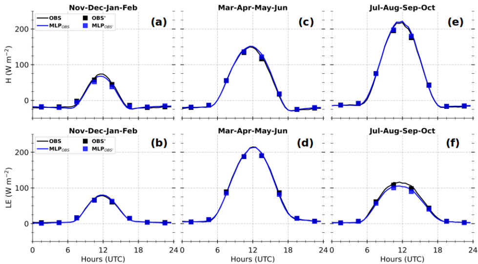
Figure 9. Composite diurnal cycles of half-hour and 3-hour observed heat fluxes (OBS and OBS' in black) and their competing MLP-based estimates (MLP OBS and MLP OBS' respectively, in blue), for H (top panels) and LE (bottom panels), by splitting the annual cycle into 3 typical sub-periods (see the text for more details). They are calculated based on diurnal cycles where at least 6 out of 8 expected OBS' are available (approximately 85% of all selected diurnal cycles).
