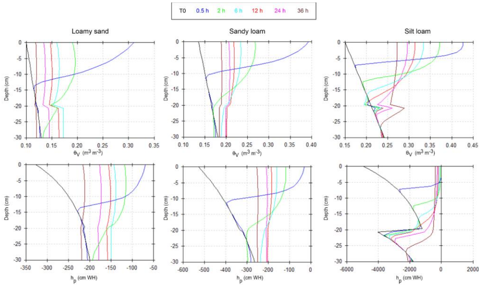
Figure A1: Simulations using HYDRUS-1D to determine when the water, added at T0, reached the lower boundary of the repacked topsoil containing ^{13}C -labeled ryegrass (at -20 cm depth). A 24-hour period after water addition was found sufficient for all three soil textures (loamy sand, sandy loam, and silt loam) to reach an approximately constant moisture level across the topsoil layer.
