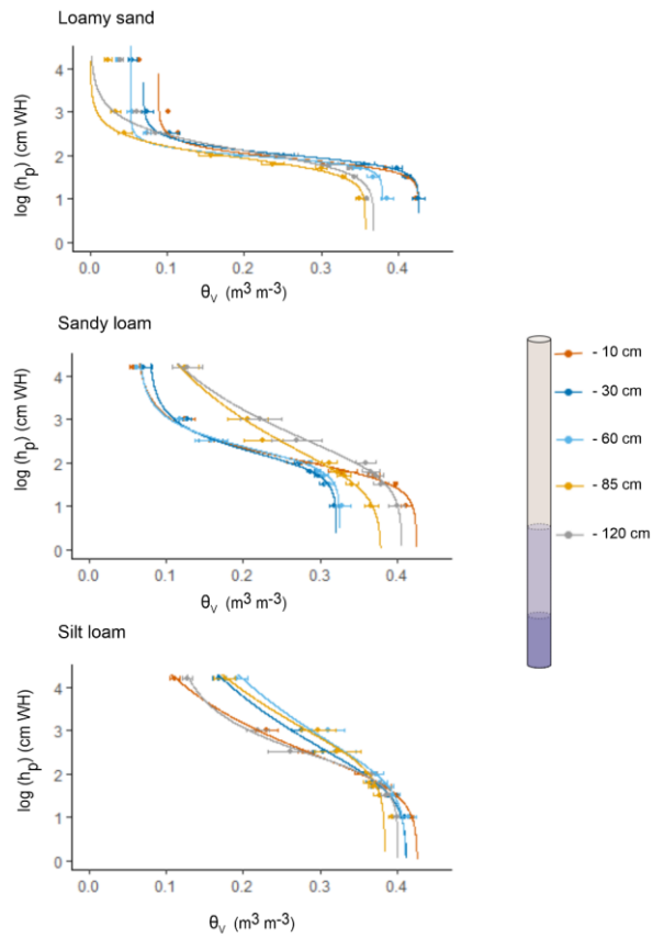
625 Figure B1: Soil water retention curves for different depths in our soil columns (n=4; except at -10 cm, n = 2).
