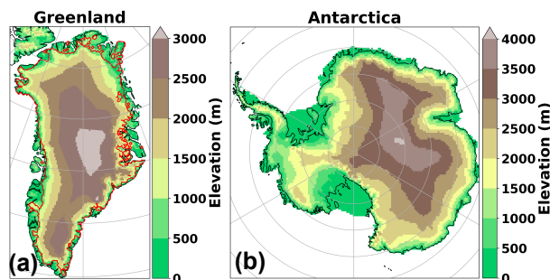
Figure 3. Topography of MAR for (a) Greenland (15km×15km) with the present-day ice sheet extent in red contour and (b) Antarctica (35km×35km).
