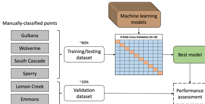
Figure 4: Schematic of the machine learning model training, testing, and validation process conducted for each satellite image product separately.
