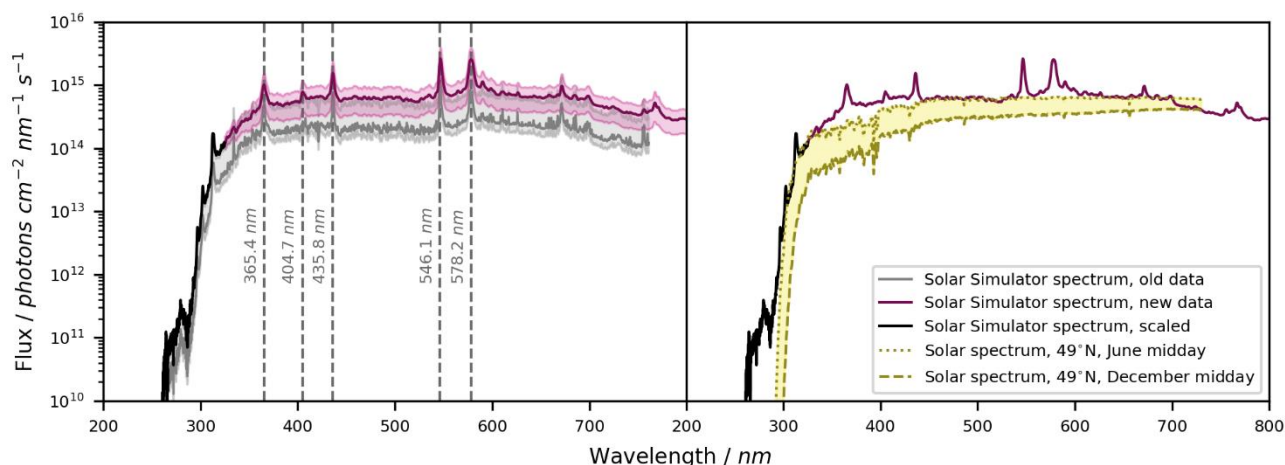
Figure 4: Solar simulator emission spectrum. The left figure shows the emission spectrum of the solar simulator (7 HMI lamps with bandpass filter) available from an old measurement (Bleicher, 2012), the newly recorded spectrum, and the scaled spectrum in the wavelength range between \lambda = 262 - 325 \text{ nm} (scaled by comparing the new data and the old data for the wavelength range \lambda = 350 - 500 \text{ nm} ). The new spectrum is shown as the mean \pm standard deviation from 30 measurements at different positions above the solar simulator. The uncertainty in the old data results from the quantification of Cl radicals used to calibrate the actinic flux. The main Hg emission lines are shown. In the right figure, the solar simulator spectrum is compared against the natural actinic flux as calculated with the TUV radiation model for 49^\circ\text{N} for midday in June and December respectively (NCAR, 2024). Figure concept inspired by Bleicher (2012).
