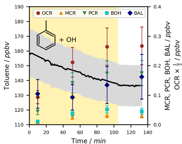
Figure 3: Exemplary time series for the OH radical-induced photooxidation of toluene at T = 298 \pm 1 \text{ K} in the absence of \text{NO}_x . The temporal profiles of toluene and its ring-retaining first generation products in experiment Tol-OH-6 are shown. Toluene was determined by PTR-ToF-MS (black line, quantification error shown as grey area), while the products were analysed using the on-line double-derivatization SPME-GC-MS method (quantification error shown as error bars). No loss corrections were applied to the depicted data. The area shaded in yellow represents the period in which the chamber was irradiated.
