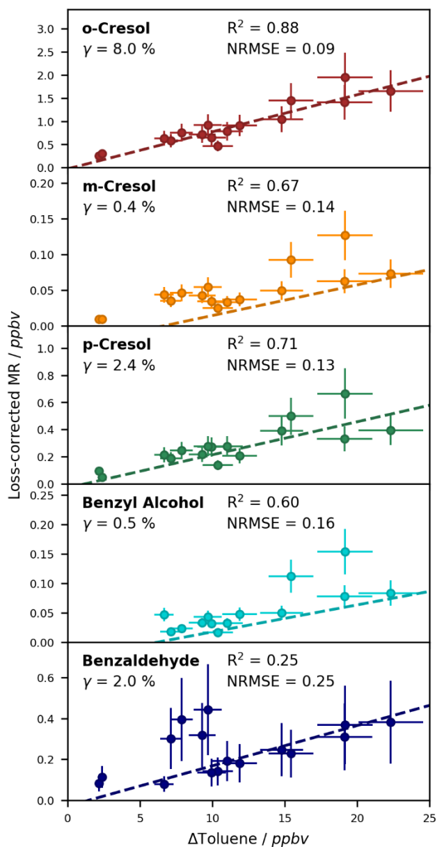
835 Figure 12: Yields of the ring-retaining first generation products of toluene, derived by linear regressions of the loss-corrected mixing ratio (including loss corrections for wall losses, photolysis, secondary OH radical reactions) against the monitored change in toluene. For each compound, the slope of the regression is equal to the formation yield. To perform the regressions, only experiments conducted at T = 298 \pm 1 K and in the absence of \text{NO}_x were used. Error bars represent the quantification error.
