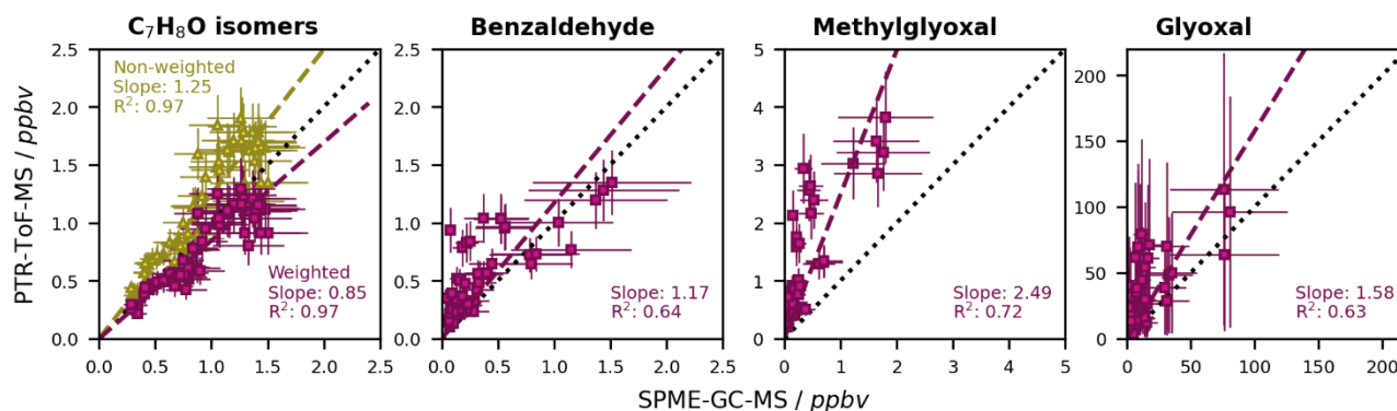
Figure 9: Comparison of the non-corrected mixing ratios of the toluene first generation products that were calibrated for both the SPME-GC-MS and the PTR-ToF-MS. The dashed black line represents a 1:1 fit. For both instruments, the mixing ratios as derived from the chamber calibration are shown. In case of the cresol isomers and benzyl alcohol, the non-weighted and weighted calibrations for the sum of the isomers are distinguished. Error bars represent the quantification error of the respective instruments. Error bars of the sum of the C_7H_8O isomers (cresols and benzyl alcohol) at the SPME-GC-MS are the weighted sum of the individual errors. The data are derived from 730 18 different experiments at different temperatures and both in the absence and presence of NO_x .
