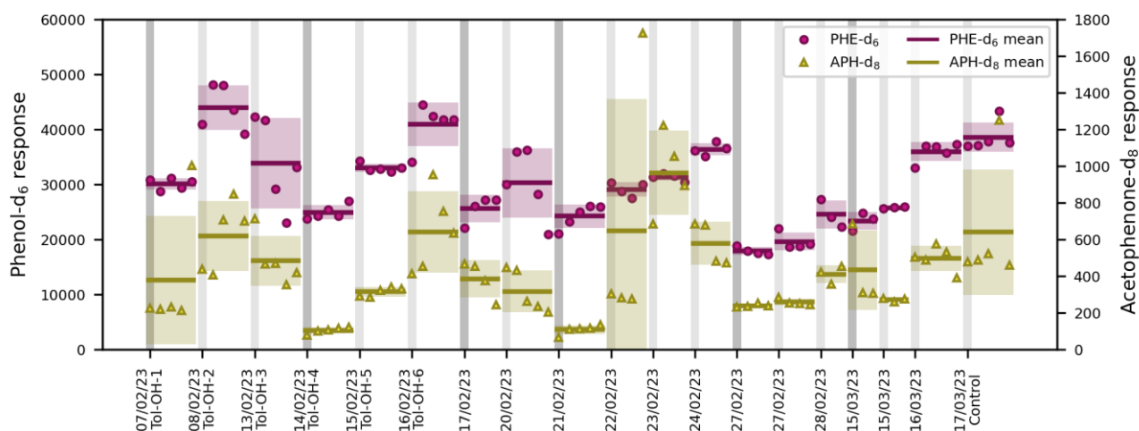
675 Figure 8: ISTD responses at the SPME-GC-MS over the entire experimental period in chronological order. Each individual marker represents one measurement of phenol-d 6 or acetophenone-d 8 , respectively. Only the experimental data are included, not the fibre conditioning and chamber cleanliness test measurements prior to each experiment. The grey vertical bars indicate the start of a new experiment. The insertion of a new SPME fibre is illustrated in dark grey. The horizontal lines show the mean value of the entire experiment, with the standard deviations included as uncertainty areas.
