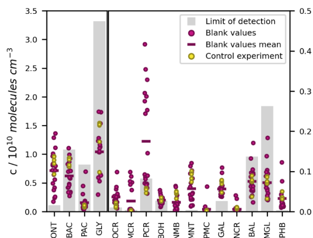
600 Figure 6: LODs, blank values, and control experiment concentrations of the toluene photooxidation products measured by SPME-GC-MS. The LODs refer to the on-line measurement from the chamber. Blank values are shown for 18 separate experiments. The measured concentrations in the toluene-free control experiment are shown without blank subtraction or further loss corrections. All values are given as concentrations in molecules \text{cm}^{-3} , because the LODs for the SPME-GC-MS were derived as fixed concentrations, whereas the corresponding mixing ratios varied between the experiments due to the ambient temperature and pressure.
