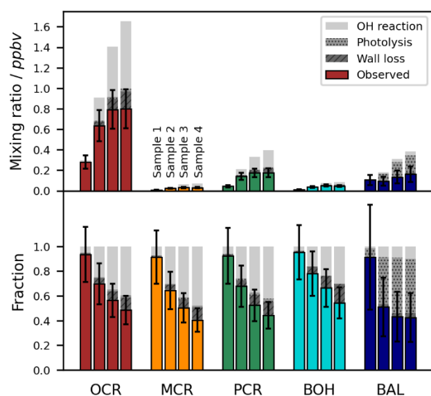
785 Figure 11: Contributions of the non-corrected data and each of the three included loss corrections (wall losses, photolysis, secondary OH radical reactions) to the final concentration. The displayed data refer to the SPME-GC-MS samples 1 to 4 in experiment Tol-OH-6 (T = 298±1 K, NO x -free). The shares of the raw data and the losses are shown on an absolute scale (mixing ratios, upper graph) and on a relative scale (normalized to the total corrected mixing ratio, lower graph). The error bars represent the compound-specific quantification errors of the non-corrected data.
