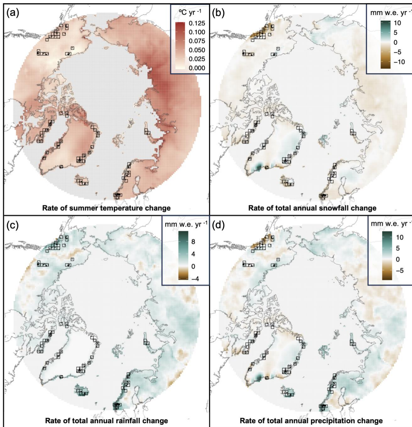
285 Figure 7. Arctic-wide changes in climate over the 1984–2022 period. (a) Rate of summer temperature change ( ^{\circ}\text{C} per year). (b) Rate of total annual snowfall change ( \text{mm w.e.} per year). (c) Rate of total annual rainfall change ( \text{mm w.e.} per year). (d) Rate of total annual precipitation change ( \text{mm w.e.} per year). In all panels, the 70, 10,000 \text{km}^2 grid cell locations are denoted
