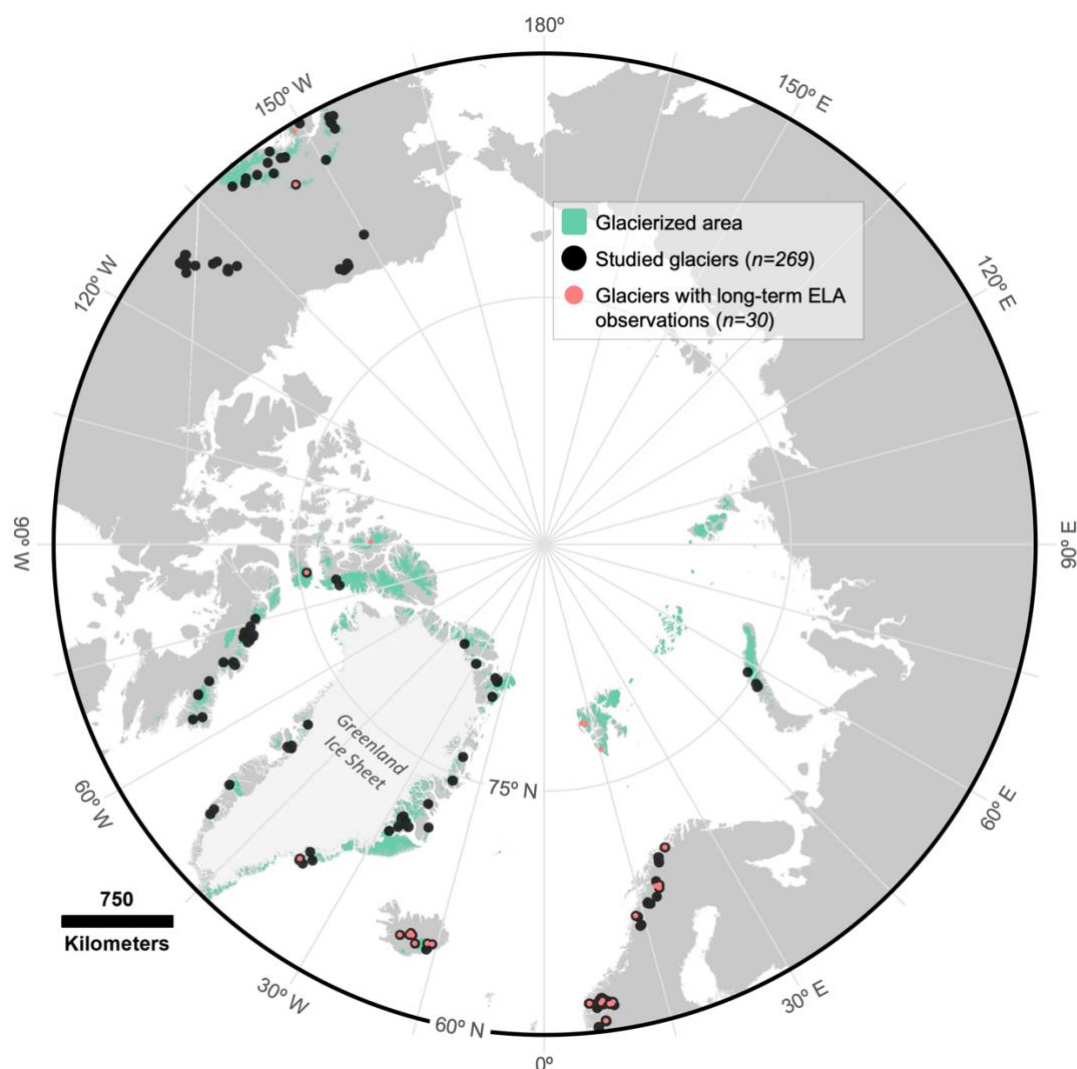
70 Figure 1. Map of the Arctic and glacier locations. Glacierized area distinct from the Greenland Ice Sheet is shown in green; the locations of the 269 land-terminating glaciers included in this study for which snowlines were digitized and analysed are denoted by black circles; and the locations of the 30 glaciers with long-term annual observations of equilibrium-line altitude (ELA) are denoted by smaller pink circles. Glacierized area from the Randolph Glacier Inventory (RGI) Version 6 (RGI Consortium, 2017).
