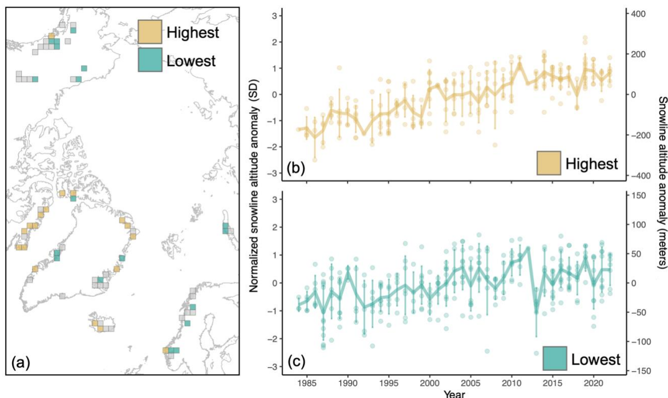
260 Figure 6. Quartile groups of grid cells that fall within the highest (yellow) and lowest (teal) 25% of the distribution of the rate of snowline altitude change (see Fig. S3). (a) Spatial distribution of grids in the quartile groups. Map is in Lambert azimuthal equal–area projection. Composite time series of snowline altitude from 1984–2022 for the mean of grid cells in (b) the highest group, and (c) the lowest group. Uncertainty is represented as the spread, equivalent to 1 SD, of all grid cells within each group (colored points) that contribute to the mean value for each year. Data are relative to the 1984–2022 mean. Note the different right–side y–axes are based on a conversion of 1 SD=129 m in panel (b) and 1 SD=48 m in panel (c).
