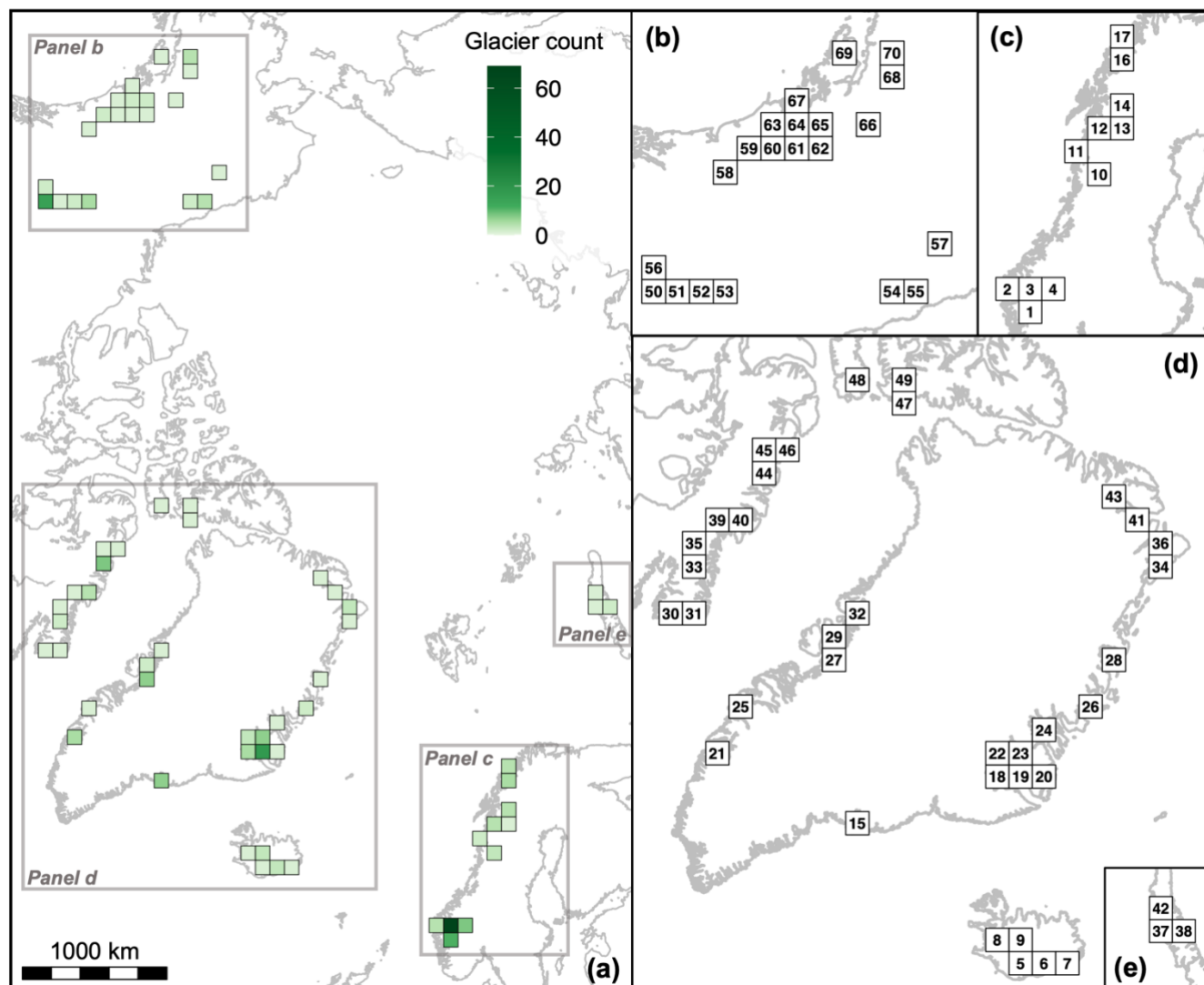
150 Figure 3. Maps of 10,000 km 2 grid cells with glacier snowline observations from this study. (a) Glacier count per grid cell. Color corresponds to the number of glaciers that fall within each grid cell. (b) Grid cell identifiers for Alaska, (c) Scandinavia, (d) Arctic Canada, Greenland, Iceland, and (e) the Russian Arctic, numbered 1–70. Maps are in Lambert azimuthal equal–area projection.
