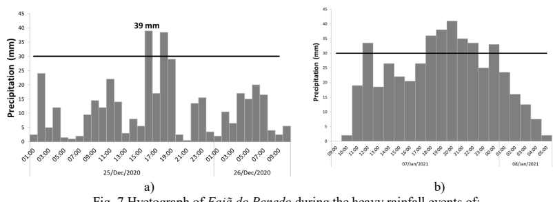
a) Fig. 7 Hyetograph of Fajã do Penedo during the heavy rainfall events of: (a) December 25, 2020; (b) January 7 and 8, 2021.
