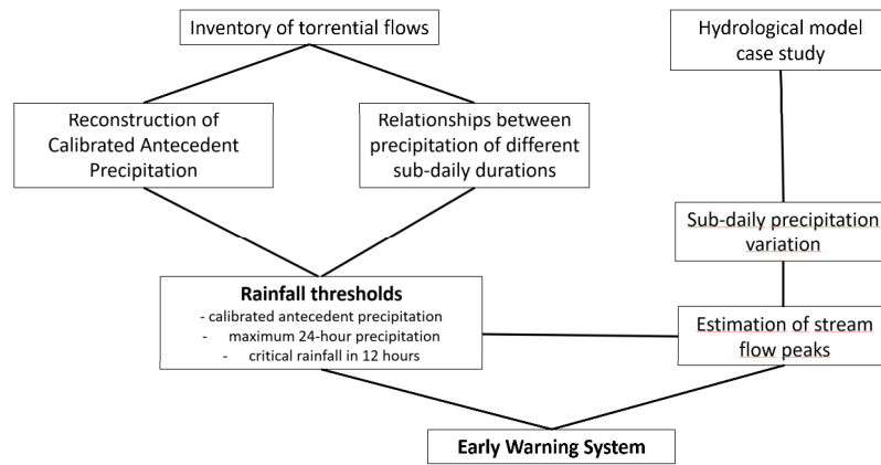
Fig. 1 Methodology for determining probable rainfall thresholds related to torrential flows and consequent peak discharges.
