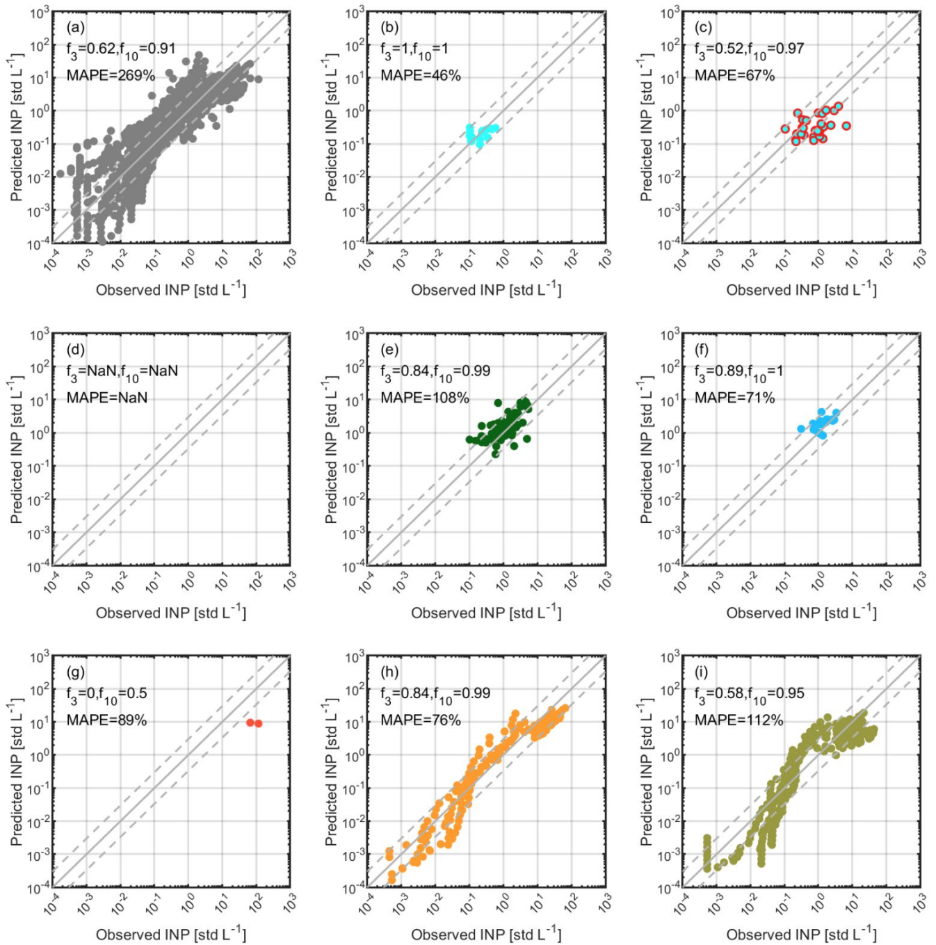
Figure S34. The same as Fig. S32 but for evaluating the predictability of Helmos Total WIBS_1 . Note that the sum of sub-datasets from panel (b) to (i) is smaller than the dataset presented in panel (a) because INP source apportionment is not available for all observations.
