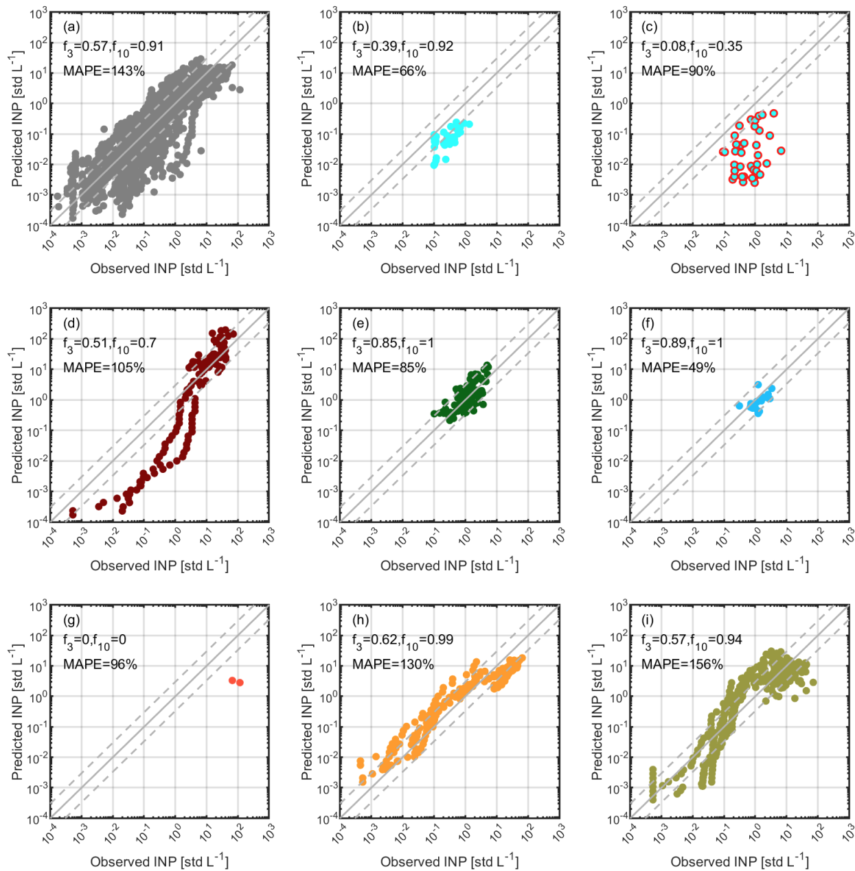
325 Figure S30. The predictability of Helmos DeMott2015 for INPs observed at (HAC) 2 from different sources when APS data are available. (a) All observations when both APS and WIBS data are available. (b) (HAC) 2 in FT under background condition. (c) (HAC) 2 in FT with precipitation/clouds. (d) North continental aerosols in PBL. No WIBS data. (e) North continental aerosols above PBL. (f) Marine aerosols above PBL. (g) South dust in PBL after marine aerosols. (h) South dust in PBL. (i) South dust with North continental aerosols. Note that the sum of sub-datasets from panel (b) to (i) is smaller than the dataset presented in panel (a) because INP source apportionment is not available for all observations.
