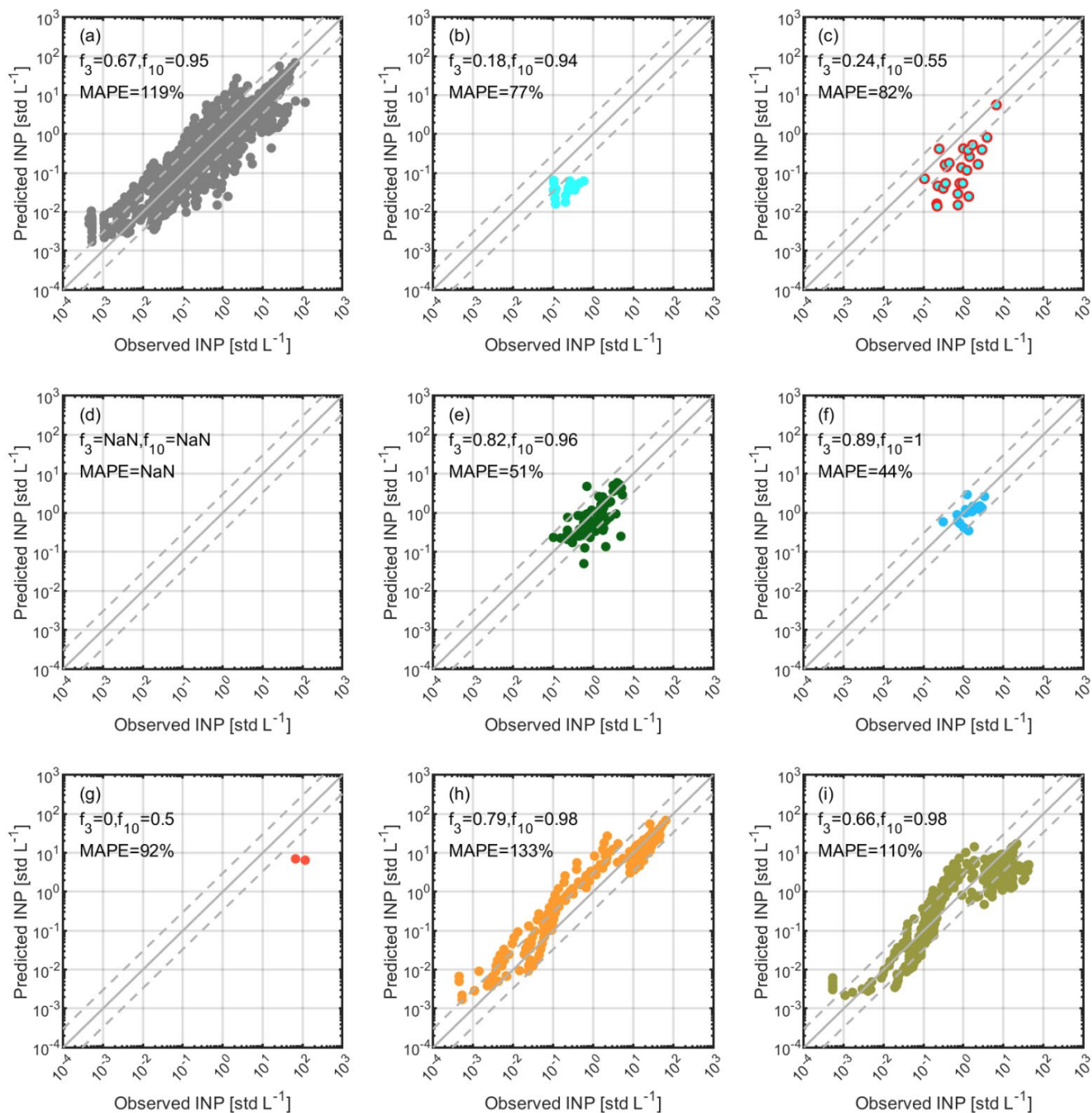
265 Figure S25. The same as Fig. S14 but for evaluating the predictability of Helmos Total WIBS_2 . Note that the sum of sub-datasets from panel (b) to (i) is smaller than the dataset presented in panel (a) because INP source apportionment is not available for all observations.
