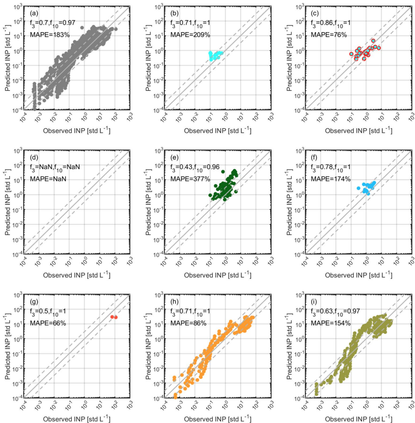
255 Figure S23. The same as Fig. S14 but for evaluating the predictability of Helmos FluowIBS. Note that the sum of sub-datasets from panel (b) to (i) is smaller than the dataset presented in panel (a) because INP source apportionment is not available for all observations.
