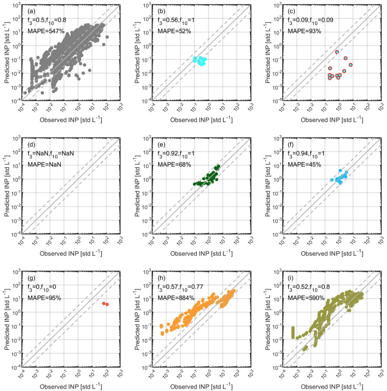
Figure S15. The same as Fig. S14 but for evaluating the predictability of DeMott2015. We note that the gap for observed INPs in panel (h) may be due to the lower estimation of INPs by INSEKT compared to PINE (see Section S3). Note that the sum of sub-datasets from panel (b) to (i) is smaller than the dataset presented in panel (a) because INP source apportionment is not available for all observations.
