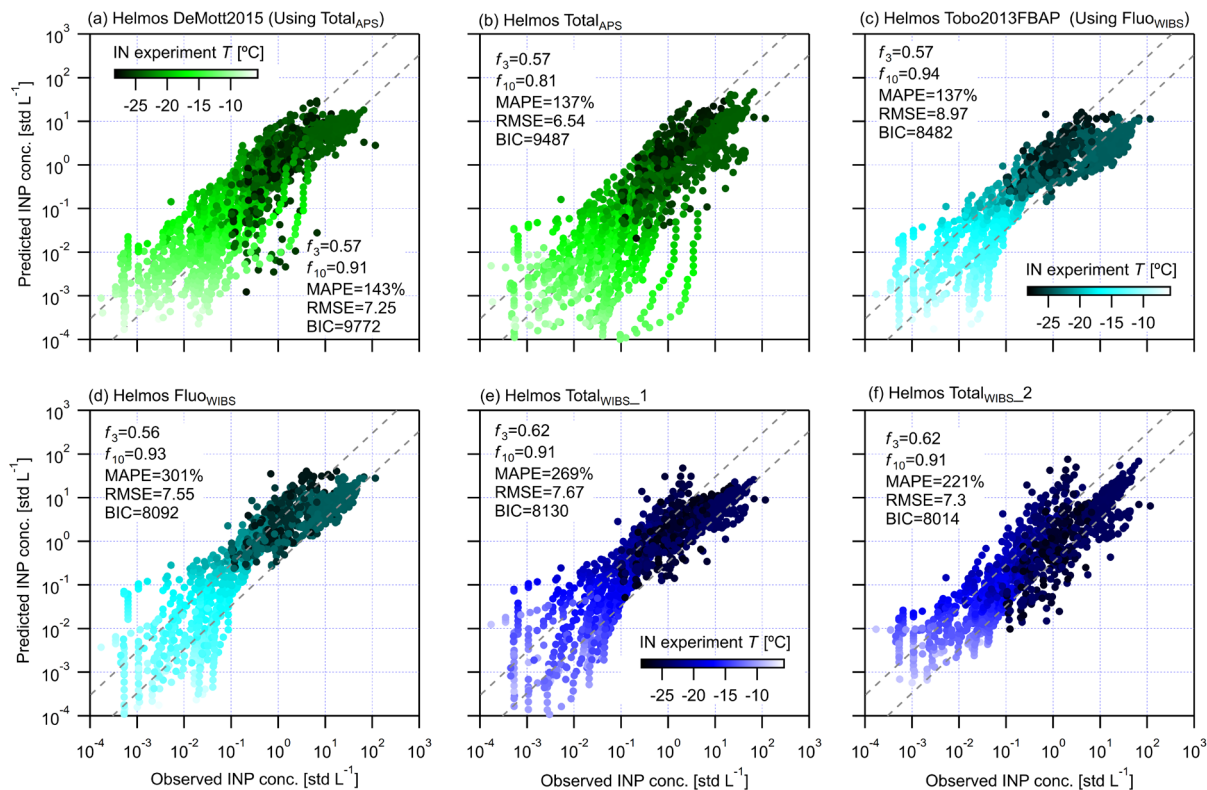
Figure S29. The predictability of different parameterization methods for all INPs observed at (HAC) 2 when APS (panel a and b) or WISB (panel c, d, e and f) data are available. (a) Helmos DeMott2015. (b) Helmos Total APS . (c) Helmos Tobo2013FBAP. (d) Helmos Fluow WIBS . (e) Helmos Total WIBS_1 . (f) Helmos Total WIBS_2 . The IN experiment temperature for observed INP data points is scaled to the colour bar. Note that parameterizations using the same aerosol properties use the same color bar. The dashed lines confine the range for observed and predicted data points within a factor of 3. The fraction of observed and predicted data points within a factor of 3 ( f_3 ) and 10 ( f_{10} ) is provided in each panel, respectively. MAPE stands for mean absolute percentage error. The results are based on observations for periods when both APS and WIBS are available, thus all parametrizations are based on the same dataset. RMSE is the root-mean-square error used as a measure of the difference between observed and predicted data. BIC is a value calculated by applying the Bayesian information criteria to evaluate the goodness of parameterizations based on the same dataset.
