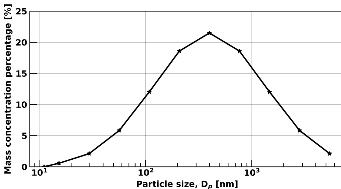
30 Figure S1. Particle size distribution in terms of particle mass concentration percentage for different size bins. The geometric mean diameter for the whole particle size distribution is 400 nm and the standard deviation is 3.3. The geometric mean diameter of each bin is indicated by the star marker.
