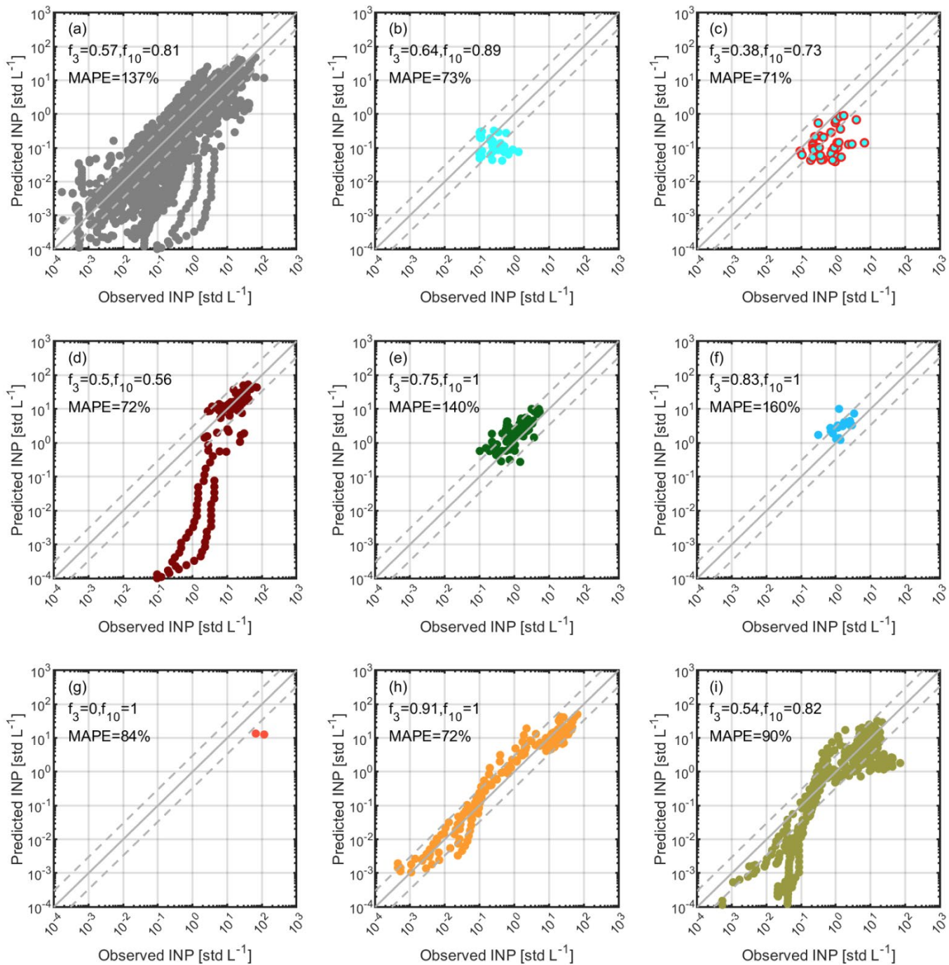
Figure S31. The same as Fig. S30 but for evaluating the predictability of Helmos Total APS . Note that the sum of sub-datasets from panel (b) to (i) is smaller than the dataset presented in panel (a) because INP source apportionment is not available for all observations.
