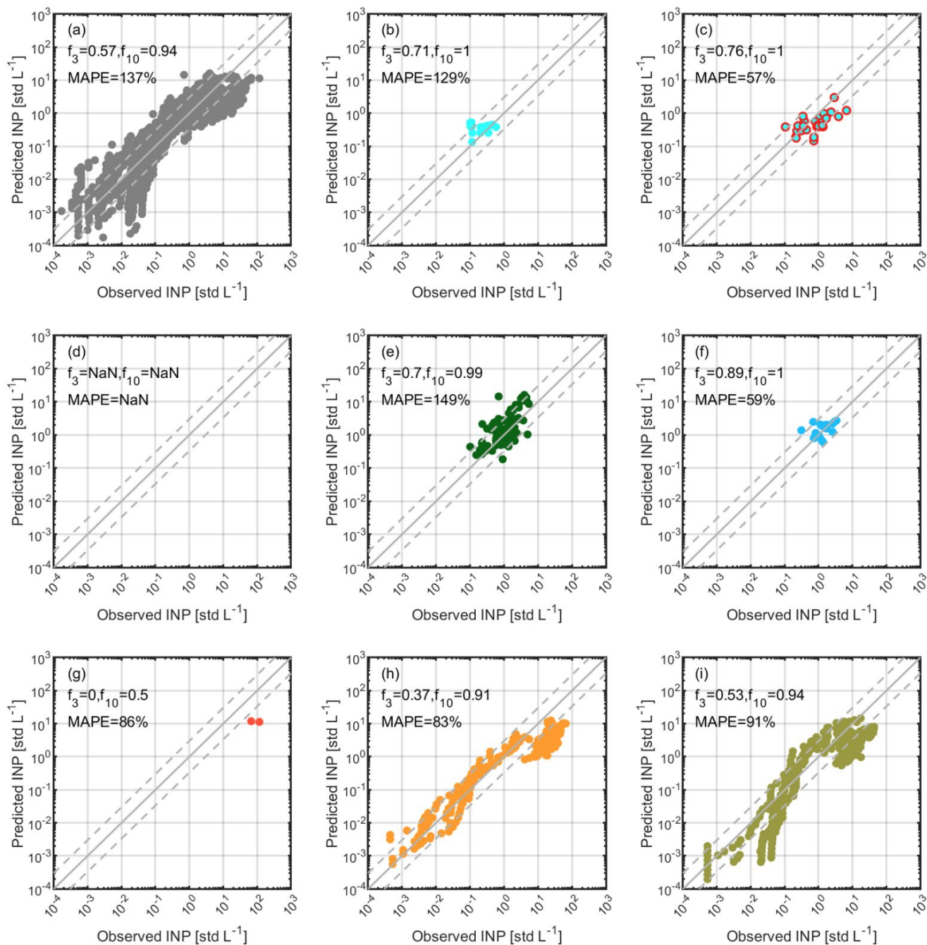
Figure S32. The predictability of Helmos Tobo2013FBAP for INPs observed at (\text{HAC})^2 from different sources when WIBS data are available. (a) All observations when both APS and WIBS data are available. (b) (\text{HAC})^2 in FT under background condition. (c) (\text{HAC})^2 in FT with precipitation/clouds. (d) North continental aerosols in PBL. No WIBS data. (e) North continental aerosols above PBL. (f) Marine aerosols above PBL. (g) South dust in PBL after marine aerosols. (h) South dust in PBL. (i) South dust with North continental aerosols. Note that the sum of sub-datasets from panel (b) to (i) is smaller than the dataset presented in panel (a) because INP source apportionment is not available for all observations.
