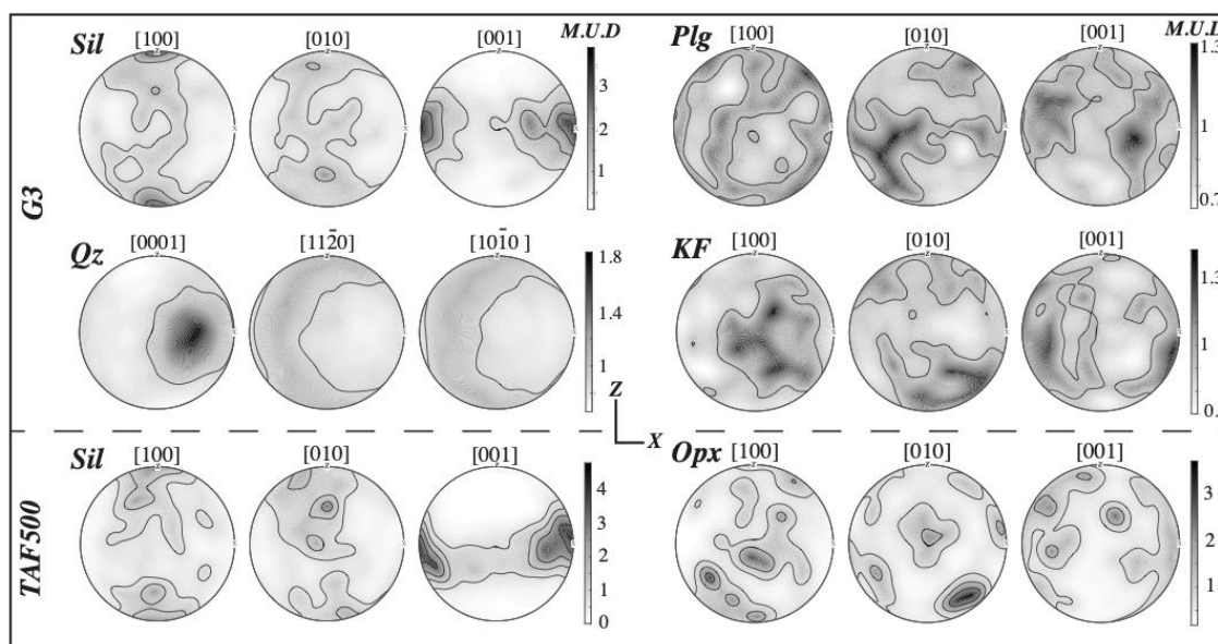
Figure 10: Representative Crystallographic Preferred Orientation (CPO) of: a) sillimanite, quartz, K-feldspar 390 and plagioclase in the quartzo-feldspathic granulite G3, b) sillimanite and orthopyroxene in the restitic granulite TAF500. Lower hemisphere stereographic projections with contours at 1 Multiple of a Uniform Distribution (MUD) intervals. The grey scale corresponds to MUD for each cell. To facilitate comparisons, CPOs have been rotated to put [001] of sillimanite in the EW direction considering that the maximum concentration of this axis is representative of the lineation. The foliation is ~EW and normal to the plane of the pole figure. In both samples, sillimanite displays a clear preferred orientation despite a weak dispersion of 395 [001] in the foliation plane. In G3 feldspars do not show any reliable preferred orientation and quartz displays a weak one without correlation with the CPO of sillimanite. In TAF500 orthopyroxene is randomly oriented. Additional data are available in supplementary data Fig. S6 and S7.
