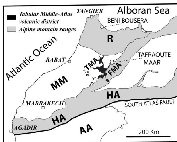
Figure 1: Sketch map showing the location of the Tafraoute maar and the Beni Bousera massif with regard to the main mountain ranges of Morocco (AA and MM: Hercynian Anti-Atlas and Moroccan Meseta; HA, FMA, TMA and R: alpine ranges of the High Atlas, Folded Middle Atlas, Tabular Middle Atlas and Rif respectively).
