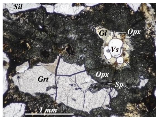
Figure 8: Microphotograph of a vesicular glass pocket (TAF501) in the center of a fibro-radiated aggregate of orthopyroxene (Opx). Gl = glass, Grt = garnet, Sil = sillimanite, Sp = spinel, Vs = vesicle.
