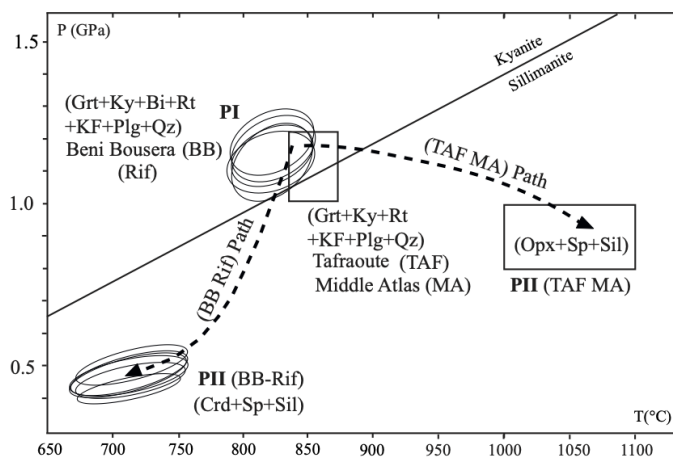
Figure 11: P-T-t diagram showing the primary (P I) and secondary (P II) parageneses of Taфраoute granulites from Middle Atlas (TAF MA) and Beni Bousera (BB-Rif). In the case of Rif granulites, the pressures and temperatures of the primary and secondary paragenesis have been determined using THERMOCALC program of Holland and Powell (1988), the ellipses correspond to 2\sigma error.
