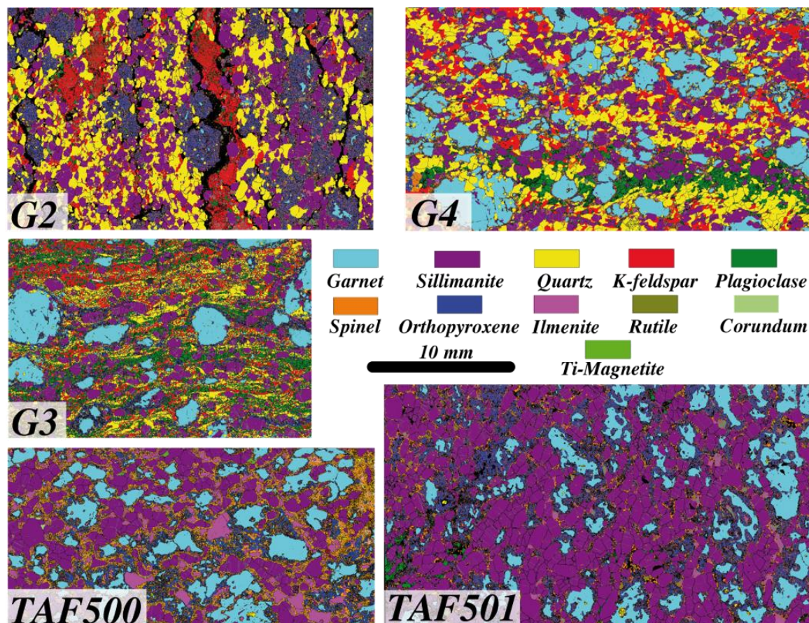
145 Figure 3: EBSD maps of the five selected granulite samples. All maps are at the same scale. The variation of the maps size only depends on the mapped area. Samples G2 and TAF500 have been cut perpendicular to the foliation and also to the lineation (YZ plane), while G3, G4 and TAF501 have been cut perpendicular to the foliation and parallel to the lineation (XZ plane). Osumilite, although present in low proportion in the quartzo-feldspathic samples, is not represented in the maps because the crystals are too small in size. Individual maps are available in supplementary 150 material.
