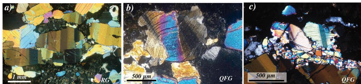
Figure 4: Photomicrograph of deformed sillimanite grains in polarized-analyzed light. (a) In TAF501, crystals showing subgrain boundaries perpendicular to the lineation and to the [001] axis of the crystals. (b) In G3, twisted crystal showing the initiation of recrystallization along the kink planes. (c) In G3, dynamic recrystallization of small new grains in parent crystals showing subgrain boundaries.
