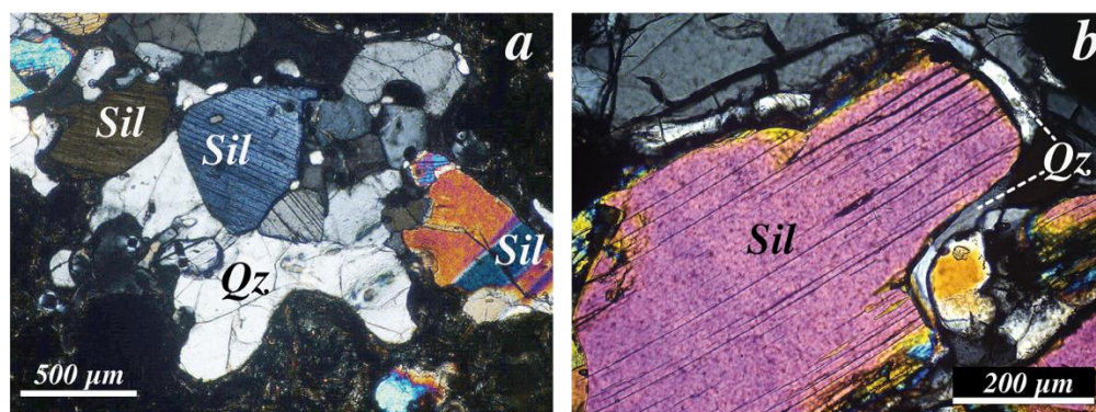
Figure 6: Photomicrograph in polarized-analyzed light of undeformed interstitial quartz crystal (a) and quartz films around sillimanite (b) in sample G4.
