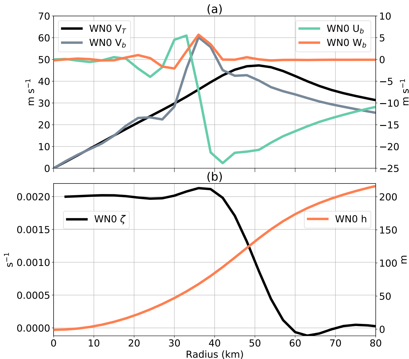
Figure 2. The initial axisymmetric radial profile of the (a) wind flow in the SBL and tangential wind in the SWM, and the (b) vorticity, and shallow water depth deviation from the mean in the SWM.
