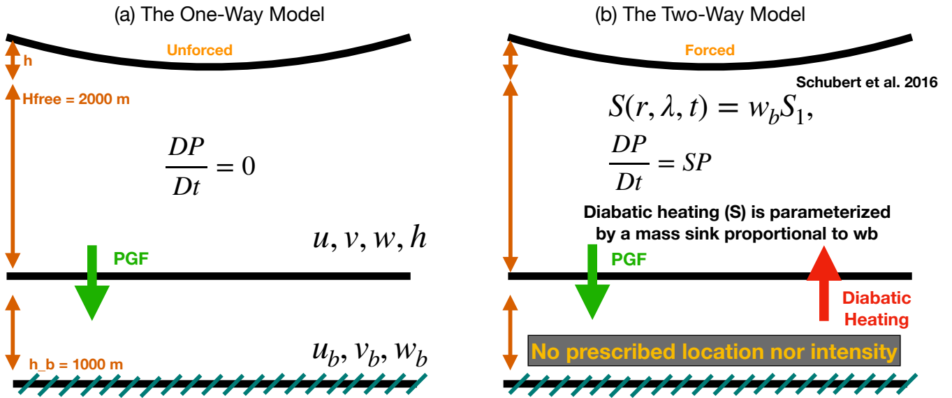
Figure 1. Schematics of the (a) One-way model and (b) Two-way model.
