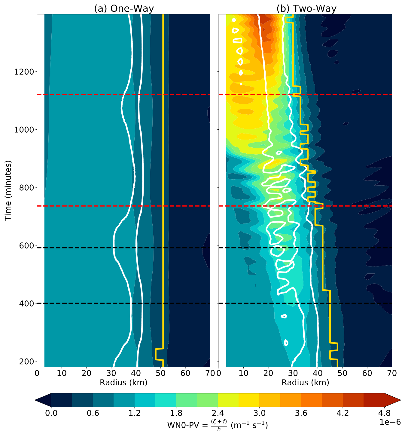
Figure 4. Time radius diagram of the wavenumber 0 potential vorticity (shading) in the SWM and the wavenumber 0 vertical velocity (white contour with an amplitude of 2 m s^{-1} in the SBL from the (a) One-way and (b) Two-way models. The yellow line denotes the RMW, and the dashed lines denote the time periods which are consistent with Fig. 3.
