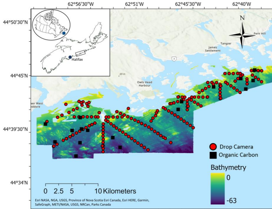
135 Figure 1. Seafloor MBES bathymetry and sample locations for the survey area at the Eastern Shore Islands, Nova Scotia, Canada (inset).
