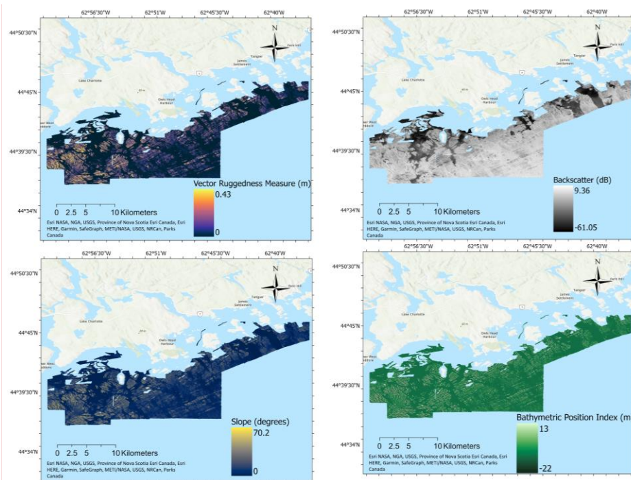
Figure 3. Backscatter, Slope, VRM and BPI data mapped in the Eastern Shore Islands study area.
