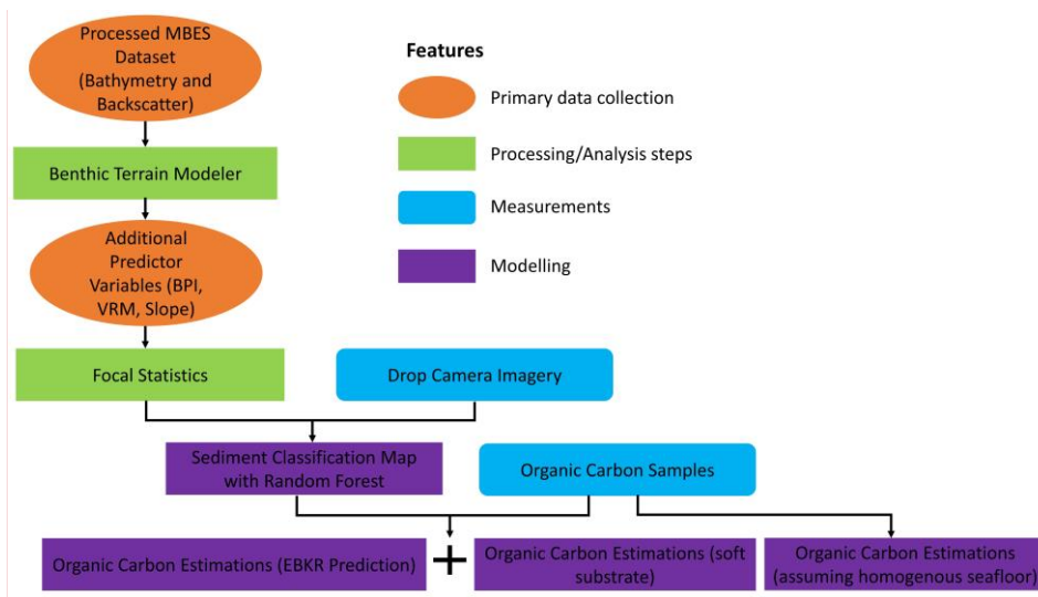
Figure 2. General analysis steps used to estimate organic carbon for four scenarios.
