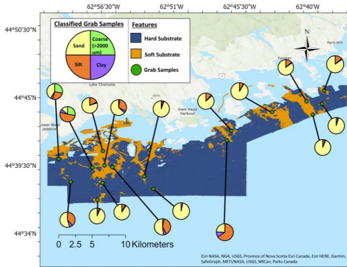
370 Figure 7. Sediment classification map indicating predicted soft (orange) and hard (blue) substrates. Pie charts depict ratios of sand (yellow), silt (orange red), clay (purple), and coarse (green) for each sediment sample collected.
