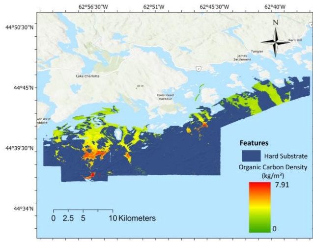
Figure 10. Spatial interpolation of OC using EBRK.
