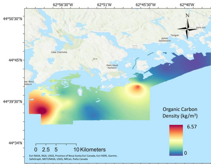
Figure 9. Spatial interpolation of OC using EBK.
