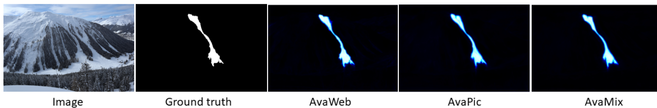
Figure 7. Example for an image from the SLF test that all three models solved well. The lighter the hue in the model predictions the higher the model certainty concerning the existence of an avalanche. In a close-up look the AvaWeb prediction exhibits more nuanced and detailed avalanche boundaries.
