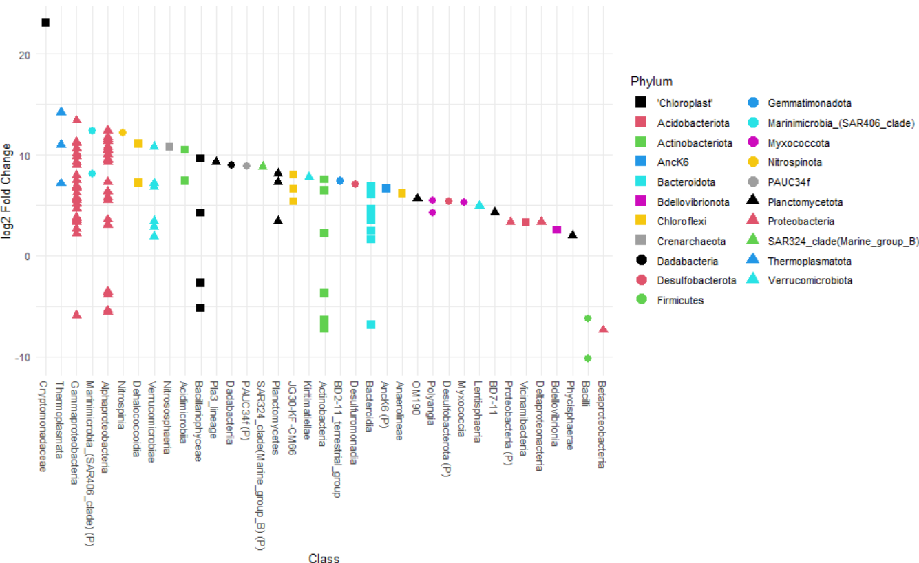
355 Figure 4. Differential abundance testing of FW dataset ASVs between provenances -Provenances using DESeq2 . The Log2 fold change in ASVs is the log-ratio of the ASV means in the water column and foraminifera. ASVs with positive Log2 fold change are significantly more abundant in the water column assemblage and ASVs with negative values indicate ASVs which are significantly more abundant in the foraminiferal assemblages. The Class, or the highest level of taxonomic assignment available for each ASV, is given on the x-axis. (P) =Phylum
