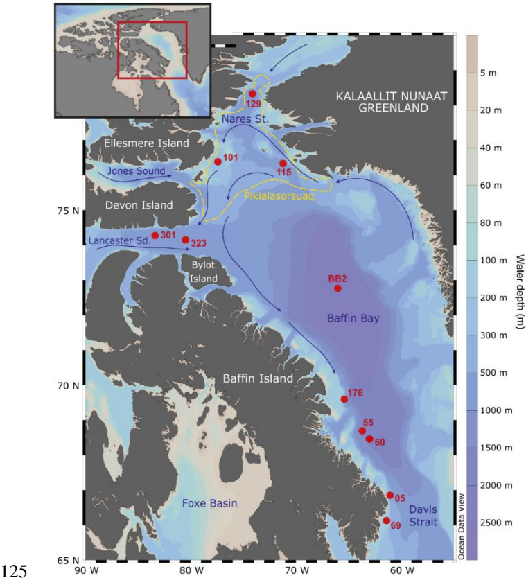
Figure 1. Map of sampling stations (numbered red spots) and the site of Pikialasorsuaq (the former ‘North Water PolynaPolynya ’ (dashed yellow line); Eegeesiak et al., 2017). Stations BB2, 101, 115, 129, 301 and 323 were part of the CCGS Amundsen ArcticNet Expedition 2017 and Stations 05, 55, 60 and 69 were part of the CCGS Hudson 2018042 Expedition 2018. Inset shows the sampling location within the wider region. The base maps were drawn in Ocean Data View v.5.6.2 (Schlitzer 2018).
