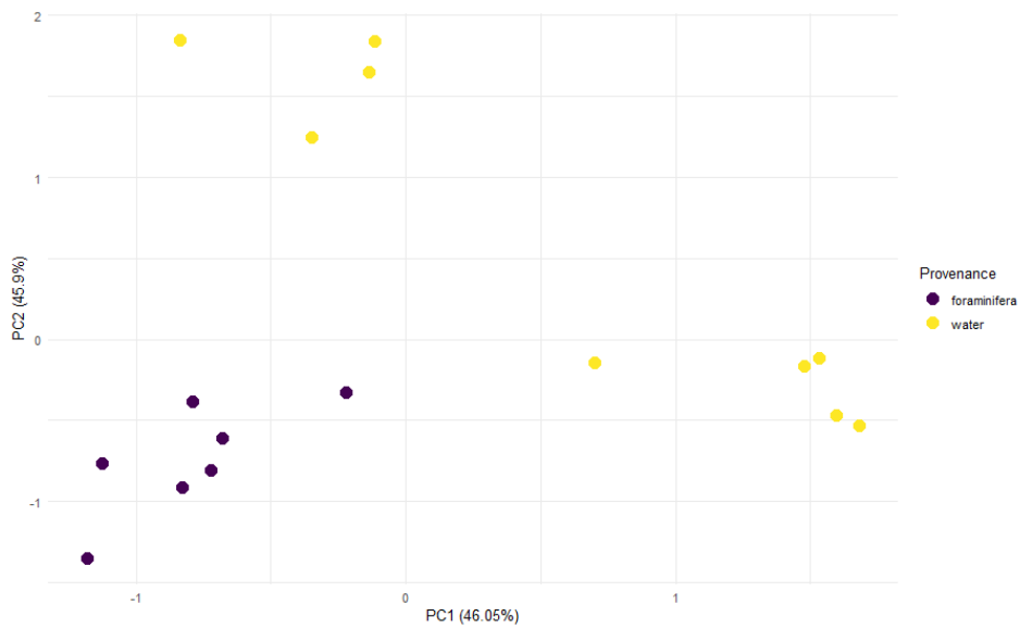
Figure A3.5 Aitchison dissimilarity PCA plot of water column (yellow) and foraminiferal samples (purple) from s Station 101. 41.7 % of the differences in ASV composition are driven by provenance Provenance ( Pr = 0.002 ; Adonis2 , Vegan ), ( P < 0.001 , (Adonis, QIIME2) ).
