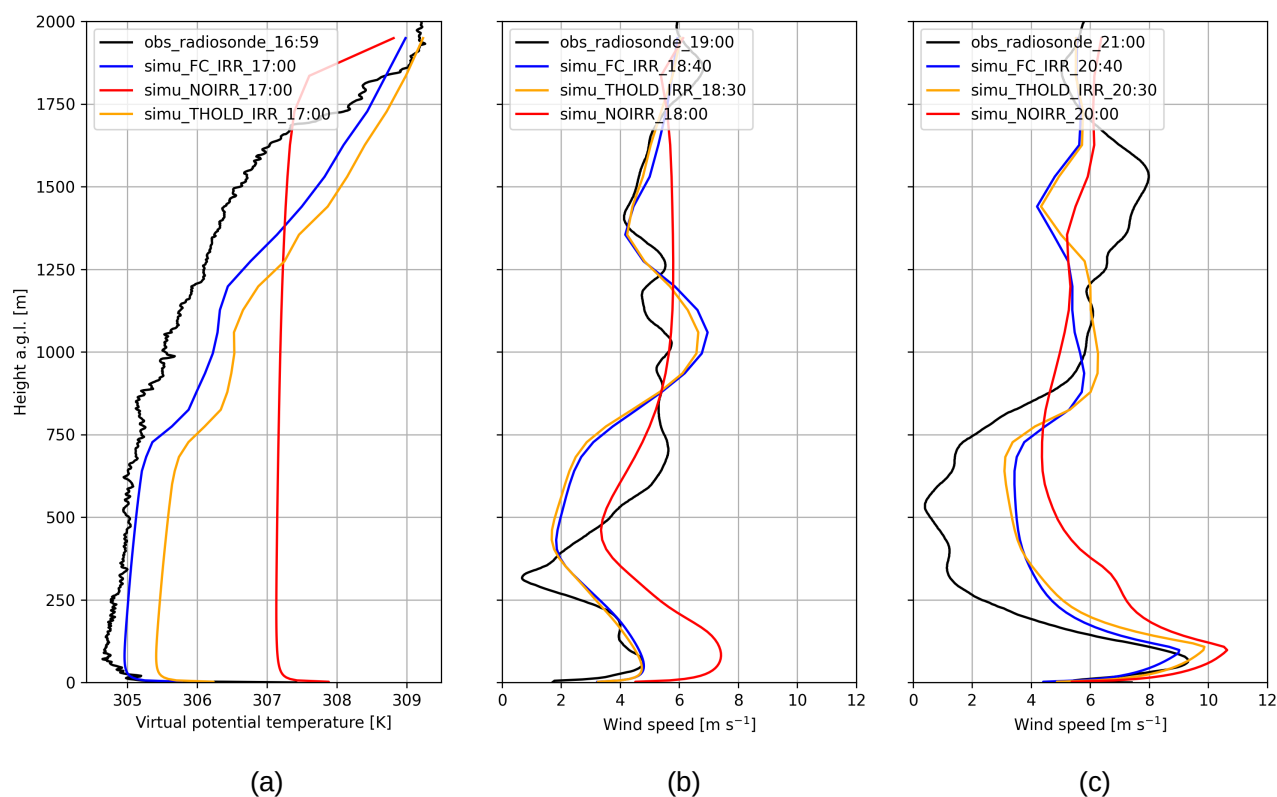
Figure 15. Vertical profile of the virtual potential temperature at Els Plans on 16 July 2021, before the Marinada arrival at 17:00 UTC (a), and of the wind speed right after the Marinada arrival (b) and 2h00 later (c). As the Marinada arrival is different in the model runs, the time considered is different for each model in (b) and (c), and the corresponding time is given in the legend.
