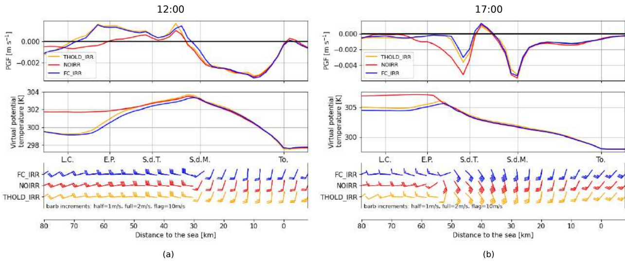
Figure 14. Pressure Gradient Force (PGF), virtual potential temperature and wind along the La Cendrosa – Torredembarra transect for 16 July 2021 at 12:00 UTC (a) and 17:00 UTC (b). The values are averaged vertically between 50 and 300 m a.g.l.
