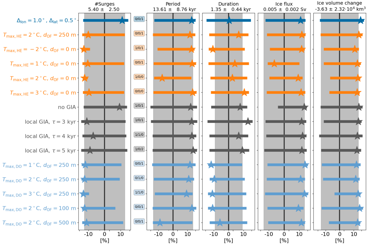
Figure 6. Percentage differences in surge characteristics compared to the reference setup for the > 2 surges sub-ensemble. The surge characteristics of the reference setup are shown in the title of each column. The shaded regions represent the MNEEs. The different colours provide visual alignment of the individual model setups. The stars and horizontal bars are the > 2 surges sub-ensemble mean percentage differences and standard deviations, respectively. The three numbers between the first and second column show the number of crashed runs, the number of runs without a surge, and the number of runs with only one surge in the comparison setup. The x-axes are logarithmic. The model setups, from top to bottom, are: \Delta_{\text{lon}} = 1^\circ , \Delta_{\text{lat}} = 0.5^\circ horizontal grid resolution, Heinrich Event shelf forcing ( T_{\text{max,HE}} = 2^\circ\text{C} , d_{\text{OF}} = 250 m), whole water column ( d_{\text{OF}} = 0 m) Heinrich Event shelf forcing with T_{\text{max,HE}} = [-2, 1, 2, 3]^\circ\text{C} (Sec. 2.3.1), no GIA model, local GIA model that is simply a damped-return to isostatic equilibrium with relaxation time constant \tau = [3, 4, 5] kyr, DO event sub-surface ocean forcing with T_{\text{max,DO}} = [1, 2, 3]^\circ\text{C} and d_{\text{OF}} = [100, 250, 500] m (Sec. 2.3.2).
