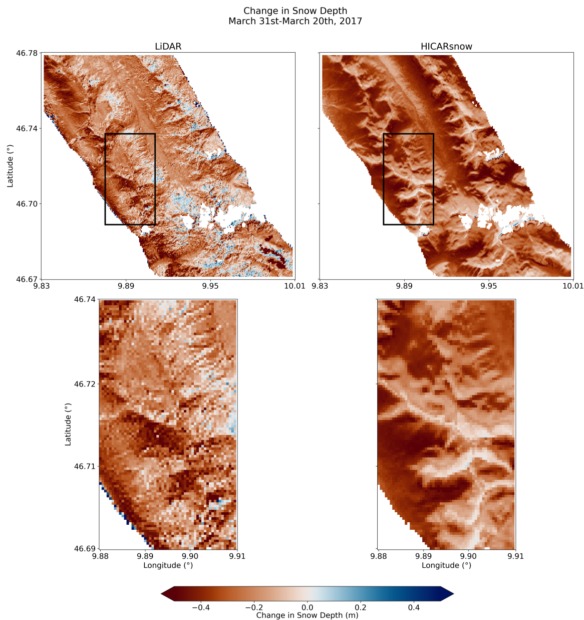
Figure 8. Maps of snow difference patterns between the two LiDAR flights at the end of March, comparing LiDAR and HICARsnow. Red colors indicate a loss of snow depth from March 20th to March 31st.
