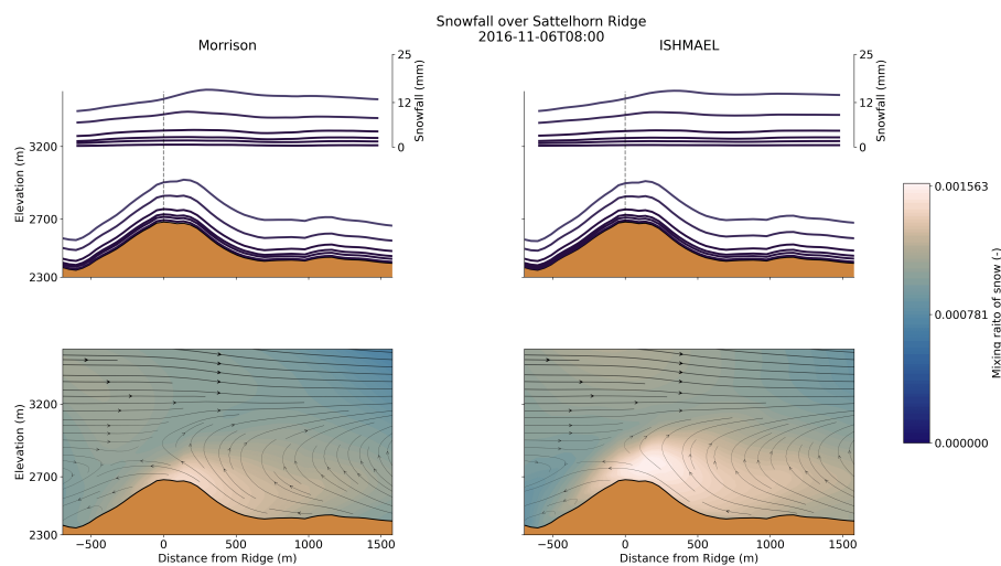
Figure 6. Demonstration of preferential deposition during a storm on November 6th, 2016. The location of the transect is shown in Fig. 1, running from the east (left) to the west (right). A vertical dashed line in the upper plot indicates the highest elevation point along the transect. The upper panels show the hourly increase in snowfall (lines in the air) and the hourly increase in snow water equivalent (lines above the terrain) since the beginning of the storm. The lower panels show wind vectors projected along this transect, and the concentration of snow particles in the air. Results using the Morrison microphysics scheme are shown on the left, and the ISHMAEL microphysics scheme is on the right.
