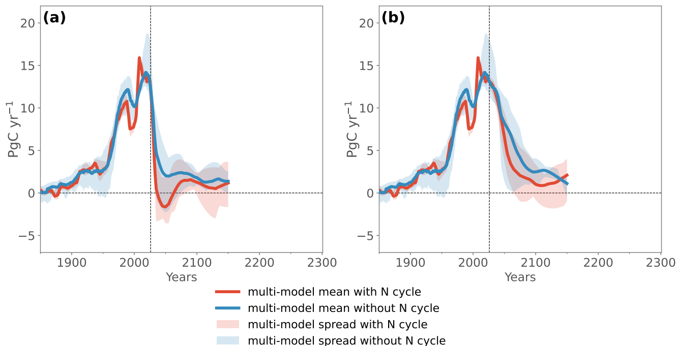
Figure B8. Simulated multi-model mean CO 2 -fe emissions for the 1.5 °C and 2.0 °C warming levels for the models that include a terrestrial nitrogen cycle (red; CESM2, EC-Earth, MIROC, MPI, NorESM2, Bern) and for the models that do not include a terrestrial nitrogen cycle (blue; NASA-GISS, GFDL-ESM2M, GFDL-ESM4, IPSL, UVic). ACCESS is not included.
