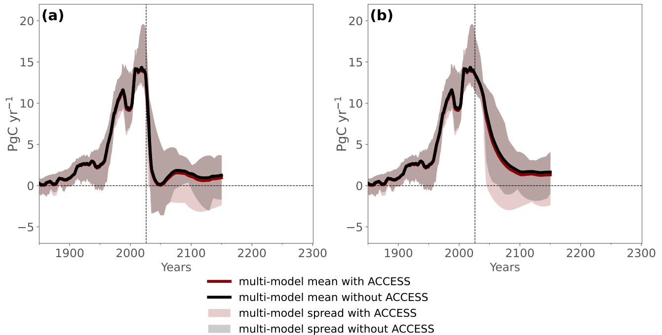
Figure B1. Simulated multi-model mean CO 2 -fe emissions for the 1.5°C and 2.0°C warming levels with and without including the ACCESS model.
