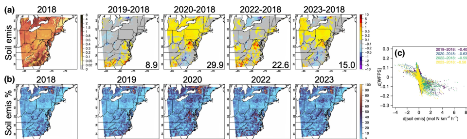
Figure 5: (a) Modeled soil NO and HONO emissions ( \text{mol N km}^{-2} \text{h}^{-1} ) and (b) soil NO and HONO emission % contributions to total anth+fire+soil \text{NO}_x emissions. Model results are averaged for MJJ 2018, shown together with the differences between MJJ of each of the following years and 2018. Numbers at the corners of the soil emission difference plots in (a) indicate the % changes relative to MJJ 2018. The scatterplot in (c) indicates relationships between the interannual differences in water-filled pore space (WFPS), whose spatial patterns are shown in Fig. S5) and soil \text{NO}_x emissions including their correlation coefficients in the upper-right legend ( p < 0.01 ).
