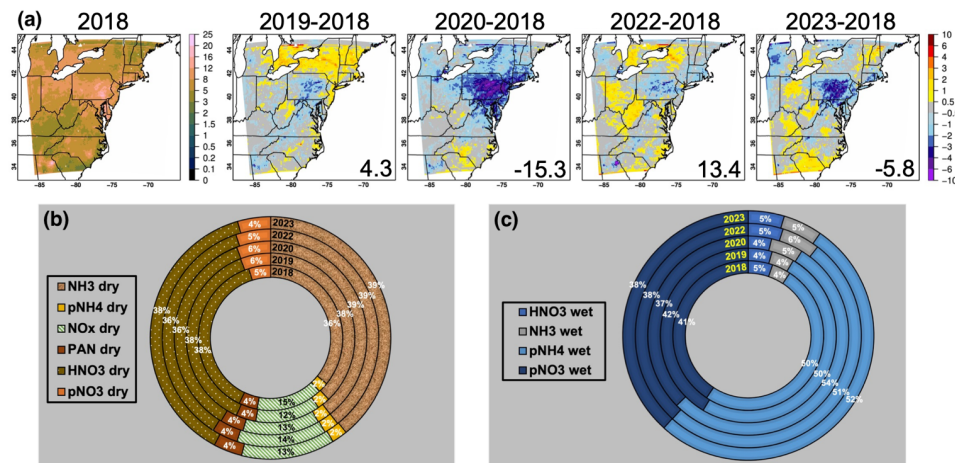
Figure 8: (a) Modeled MJJ 2018 total Nr deposition overland and differences between MJJ of each of the following years and 2018 in \text{kg N ha}^{-1} \text{ a}^{-1} ; and speciation of modeled (b) dry and (c) wet deposition fluxes by year, where prefix “p” indicates particle.
