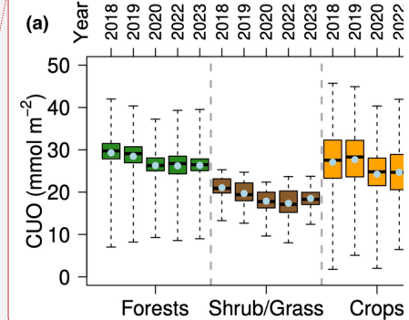
Figure 12: Box-and-Whisker plots of (a) CUO and (b) mean total Nr deposition fluxes for MJJ 2018–2023 by the grouped surface types defined in Fig. 1b.
