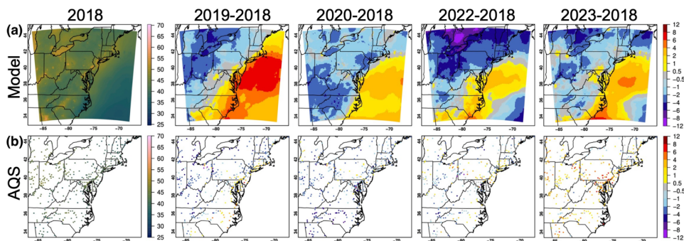
1335 Figure 10: (a) WRF-Chem modeled and (b) AQS daytime surface O 3 . Results are averaged for MJJ 2018, shown together with the differences between MJJ of each of the following years and 2018, all in ppbv. Observations from the AQS sites having <10% missing data for each year were used for evaluation. Model vs. AQS RMSEs (number of grids having collocated observations) for 2018, 2019, 2020, 2022, 2023 are 5.6 (375), 6.5 (377), 5.9 (373), 4.8 (370), and 4.0 (381), respectively.
