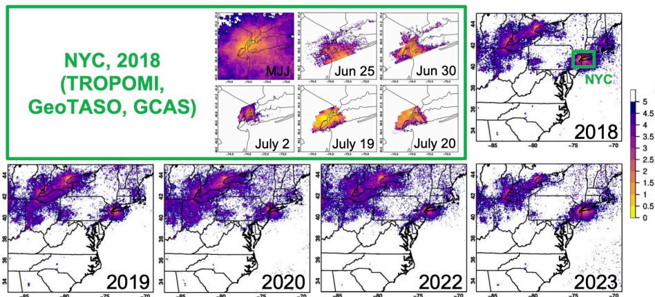
1330 Figure 9: TROPOMI (MJJ 2018–2023), GeoTASO (25 and 30 June 2018) and GCAS (2, 19 and 20 July 2018) HCHO/NO 2 ratios. GeoTASO and GCAS both took measurements over the Greater New York City (NYC) several times during the sampling days which indicate subdaily variability in HCHO, NO 2 and their ratio. Their measurements closest to 19 UTC are used here.
