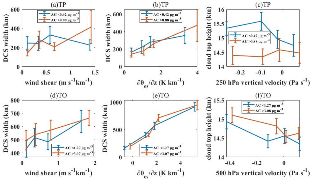
Figure 7: Bin-averaged wind shear ( \text{m s}^{-1}\text{km}^{-1} ; a, d), the vertical gradient of the saturated equivalent potential temperature \partial\theta_{es}/\partial z ( \text{K km}^{-1} ; b, e) and vertical velocity ( \text{Pa s}^{-1} ; c, f) with DCSs width (km) and cloud top height (km) from different subregions. The blue lines represent the results at weak aerosol loading (less than 30th percentiles) and the red lines represent the results at strong aerosol loading (more than 70th percentiles). The error bars represent the standard error of the mean (SEM=standard error / \sqrt{n} ). 525
