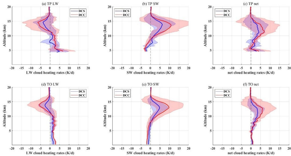
460 Figure 6: The mean vertical profiles of longwave (a, d), shortwave (b, e), and net (c, f) cloud radiative heating rates (CRH) ( K d^{-1} ) in the TP and TO. The red lines represent the results of DCCs and the blue lines represent the results of DCSs. The shadow range represents the standard deviation.
