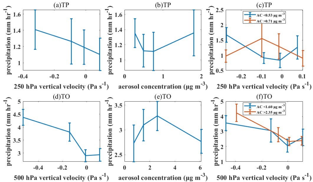
Figure 8: Bin-averaged vertical velocity (Pa s -1 ; a, d) and aerosol concentration (μg m -3 ; b, e) with precipitation (mm hr -1 ) from different subregions and the relationship between vertical velocity and precipitation under different aerosol conditions (c, f). The blue lines represent the results at small aerosol loading (less than 30th percentiles) and the red lines represent the results at large aerosol loading (more than 70th percentiles). The error bars represent the standard error of the mean (SEM=standard error / \sqrt{n} ).
