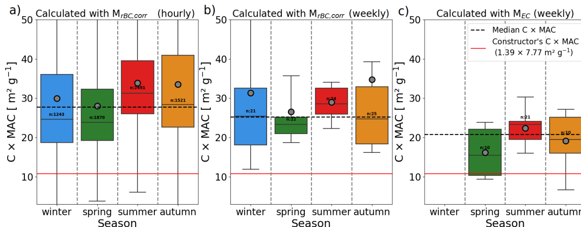
Figure 9. C \times MAC as a function of the season calculated with a) M_{rBC,corr} in an hourly basis, b) M_{rBC,corr} averaged over the sampling period of the Sunset, and c) M_{EC} , excluding TC loading < 25 \mu\text{gC cm}^{-2} . Constructor's values are represented with a red solid line while median values are represented with a black dashed line. For b), the median is calculated excluding winter's value to be in agreement with c). Boxes, lines, black dots and whiskers indicate 25 th percentile, 75 th percentile, median, mean, 10 th percentile and 90 th percentile, respectively.
