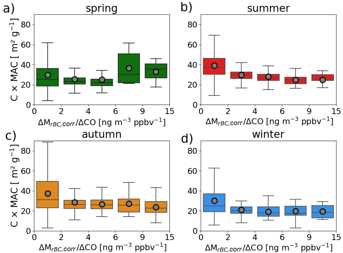
Figure 10. a) to d) C \times \text{MAC} as a function of the \Delta M_{rBC,corr}/\Delta \text{CO} emission ratio for spring, summer, autumn and winter, respectively. Boxes, lines, black dots and whiskers indicate 25 th percentile, 75 th percentile, median, mean, 10 th percentile and 90 th percentile, respectively.
