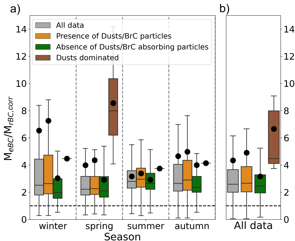
Figure 11. M_{eBC}/M_{rBC,corr} as a function of the dominant aerosol type a) as a function of the season and b) over the 2-year measurement campaign. Boxes, lines, black dots and whiskers indicate 25 th percentile, 75 th percentile, median, mean, 10 th percentile and 90 th percentile, respectively.
