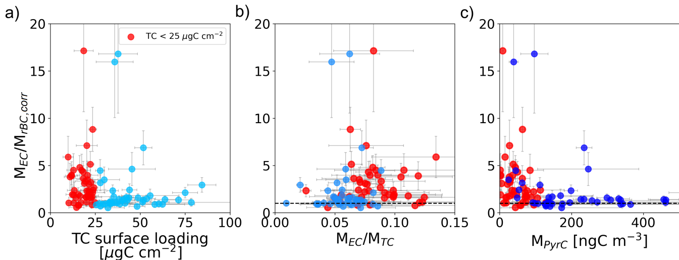
Figure 5. M_{EC}/M_{rBC,corr} as a function of a) Total Carbon surface loading, b) M_{EC}/M_{TC} and c) M_{PyTC} . Points have a weekly time resolution. Red dots highlights data where the TC loading is under 25\mu\text{gC cm}^{-2} . Error bars represent the uncertainties for each variable considering the Sunset measurements uncertainty and the SP2 ones marked in Table 1.
