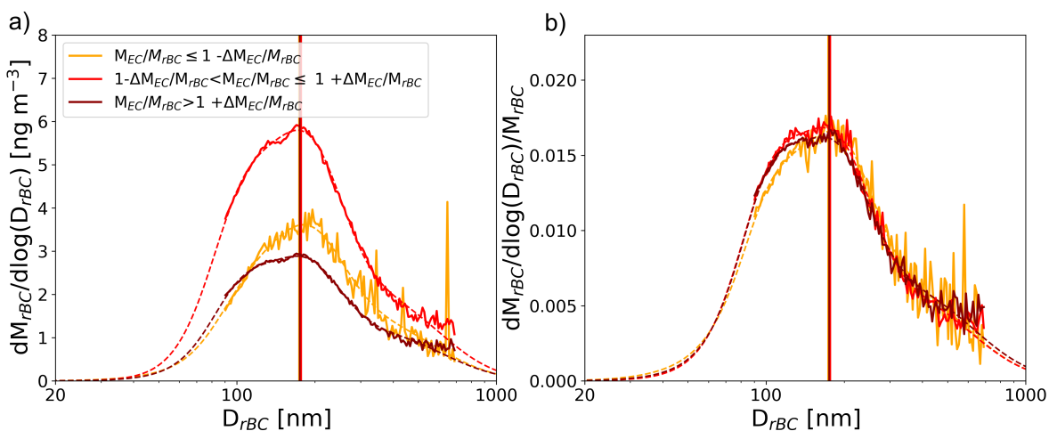
Figure 8. a) Mass size distribution of rBC core measured by the SP2, colored by M_{EC}/M_{rBC,corr} ranges of values. b) is the same as a) but normalised by the total rBC mass. Vertical lines highlight geometrical diameter corresponding to the color of the M_{EC}/M_{rBC,corr} range.
