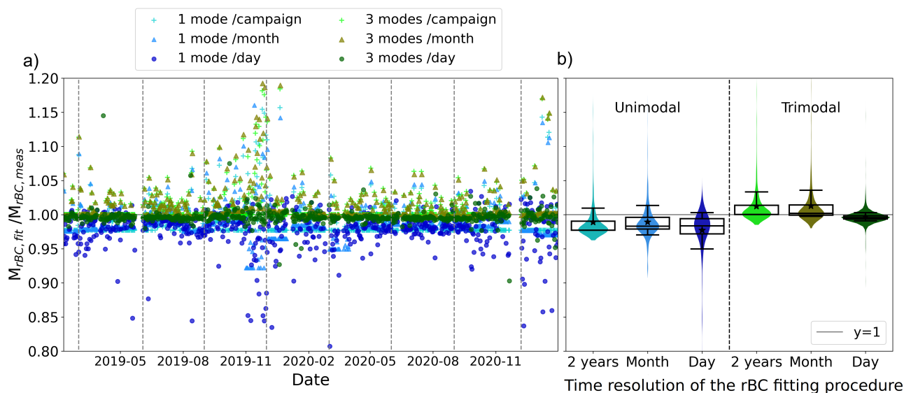
Figure 2. a) Time series and b) statistics of M_{rBC,fit}/M_{rBC,meas} calculated between 1 and 1000 nm when representing the rBC size distribution with one (lightblue to darkblue) or three (light green to darkgreen) modes and when fitting on the mean campaign (crosses), monthly (triangles) or daily (plain circles) size distribution. Violin plot represent the probability density function of M_{rBC,fit}/M_{rBC,meas} . Boxes and whiskers represent the 25 th , 75 th , 10 th and 90 th percentiles. Lines and stars show median and mean values.
