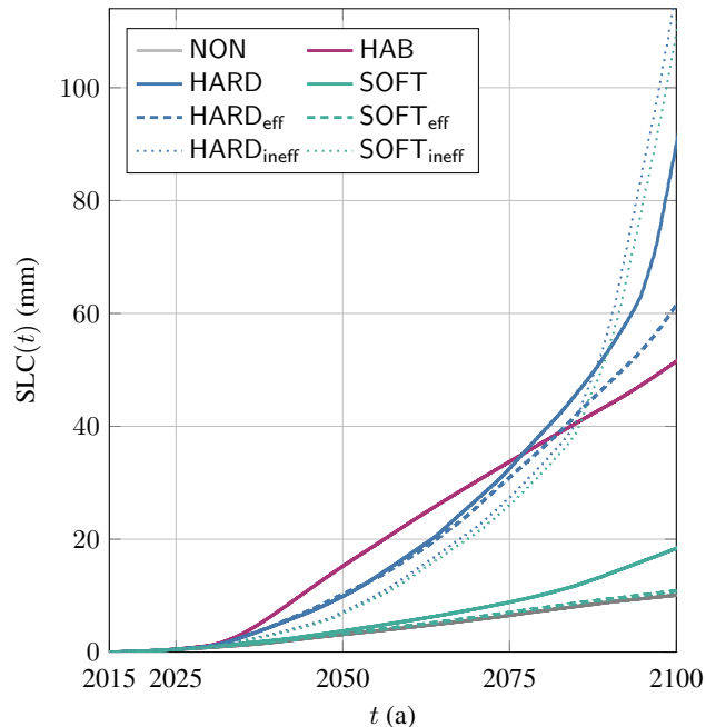
(b) Sea-level contribution from Thwaites Glacier from 2015 to 2100 under constant present-day climate conditions (atmospheric and oceanic) for the NON (grey), HAB (purple), HARD (blue), SOFT (green), HARD efficient (blue dashed line), HARD inefficient (blue dotted line), SOFT efficient (green dashed line) and SOFT inefficient (green dotted line).
