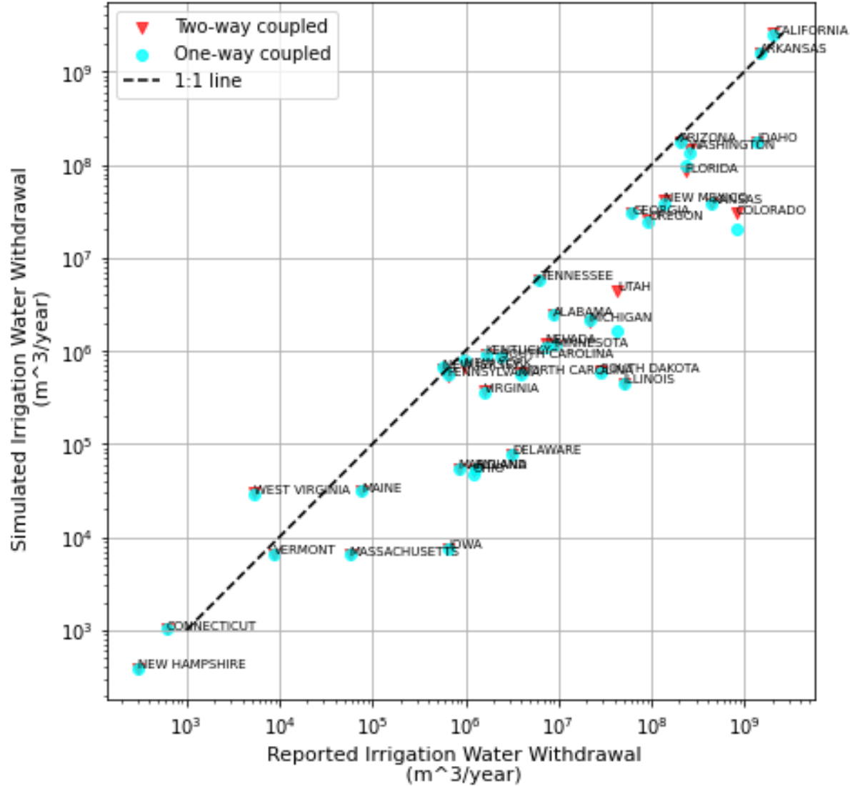
Figure 10: Spatial variation of one-way and two-way irrigation water withdrawal compared with USGS-reported water withdrawal data per state for all crops across the CONUS region with a logarithmic scale
