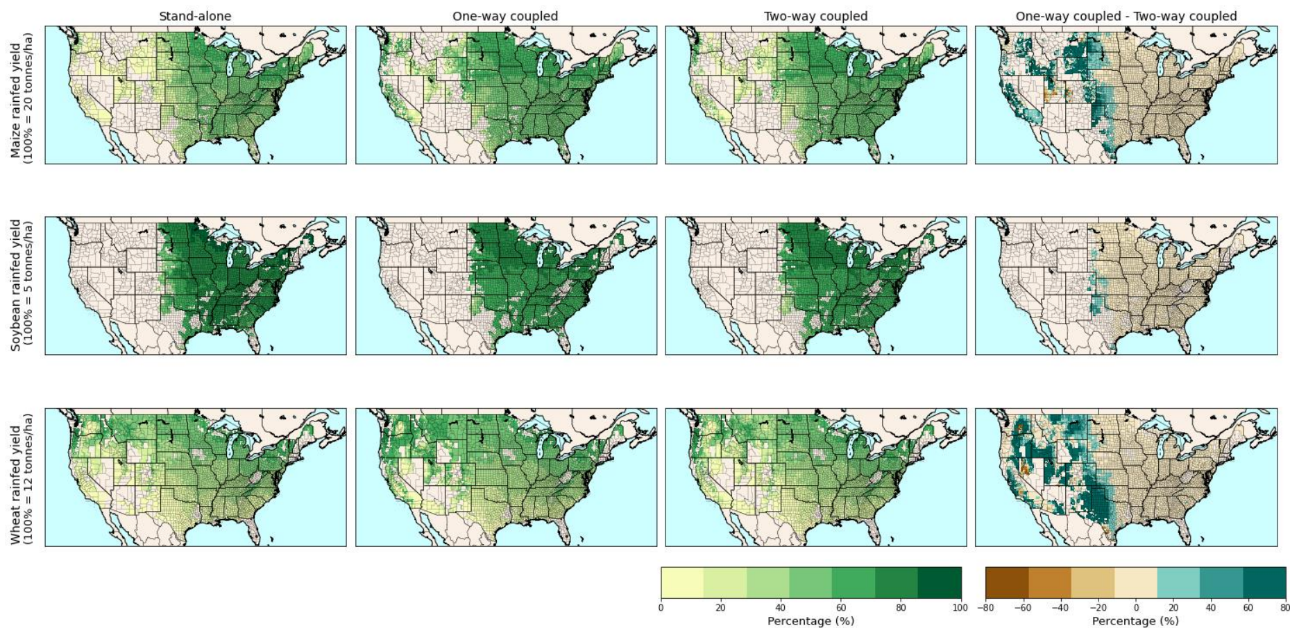
Figure-5 7: Mean rainfed crop yields for maize, soybean, and wheat within CONUS as obtained from stand-alone , one-way and two-way coupled simulations and differences between one-way and two-way coupled simulation for 1979-2019. Legend in % of values shown on the y-axes
