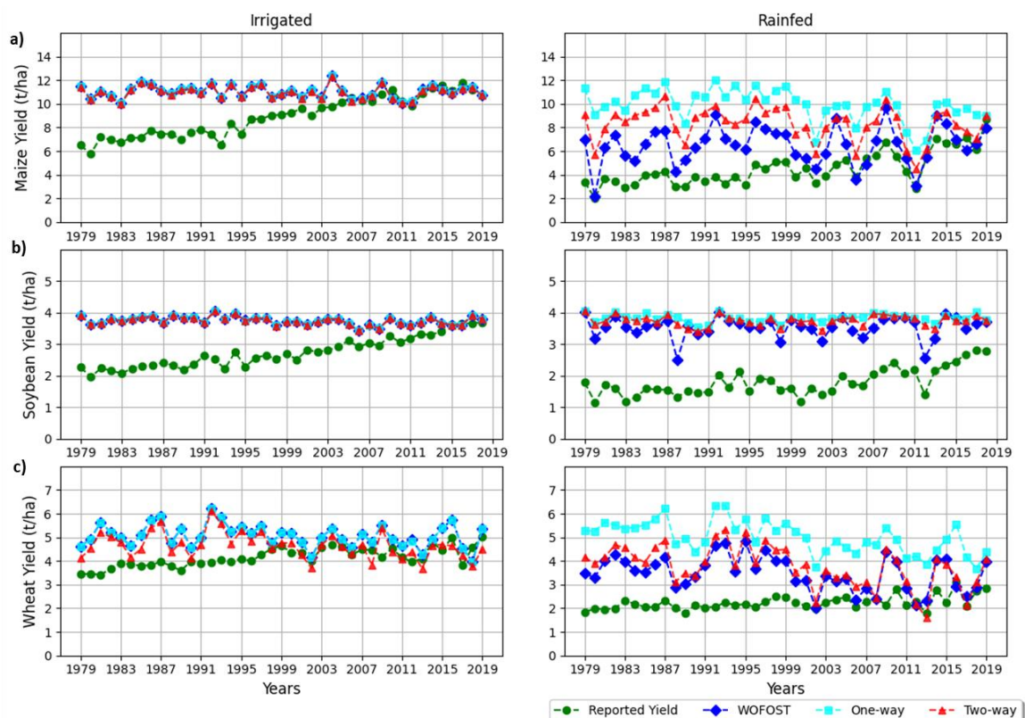
Figure 42: Temporal analysis of irrigated and rainfed crops of a) maize, b) soybean and c) wheat for the years 1979 to 2019 of a CONUS region
