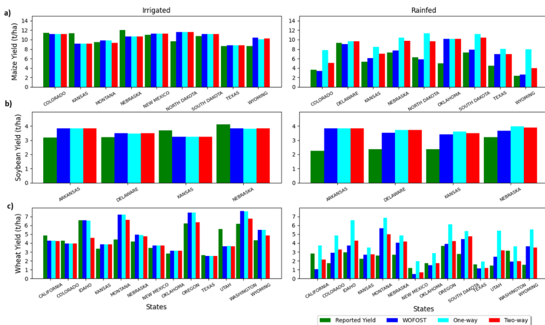
Figure 53: Spatial (i.e. state level) analysis of irrigated and rainfed crops of a) maize, b) soybean and c) wheat for the years 2006 to 2019 for the CONUS region.
