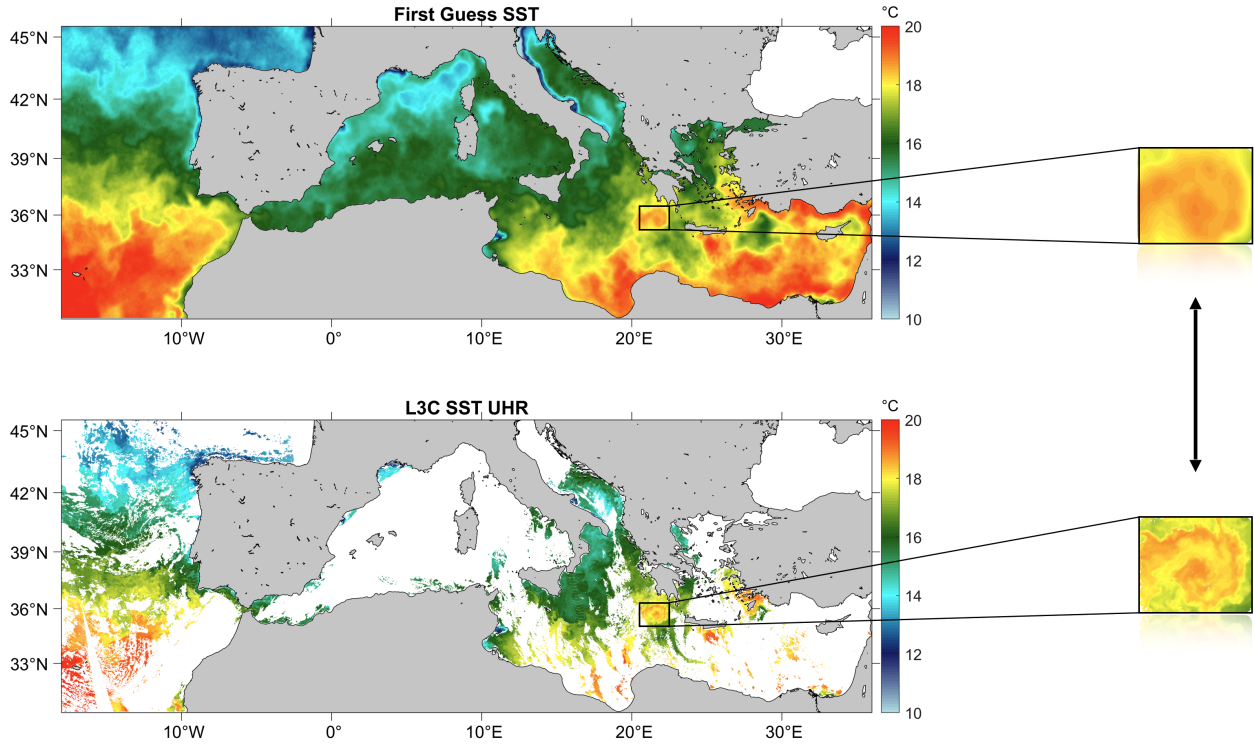
Figure 2. On the left the SST First Guess map used to extract the input tiles (top) and the SST L3C target image (bottom) on 4th January 2020. On the right an example of an extracted tile used for the training and test datasets.
