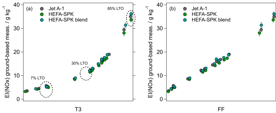
380 Figure 7: EI(NO x ) from ECLIF3-2 ground-based measurements behind the Airbus A350-941 with Rolls-Royce Trent XWB-84 engines versus T3 (referenced to 60% RH, (a)) and FF (fuel flow) (b) for Jet A-1, HEFA-SPK and Blend. Values on the x-axis are undisclosed. Black circles indicate LTO points.
