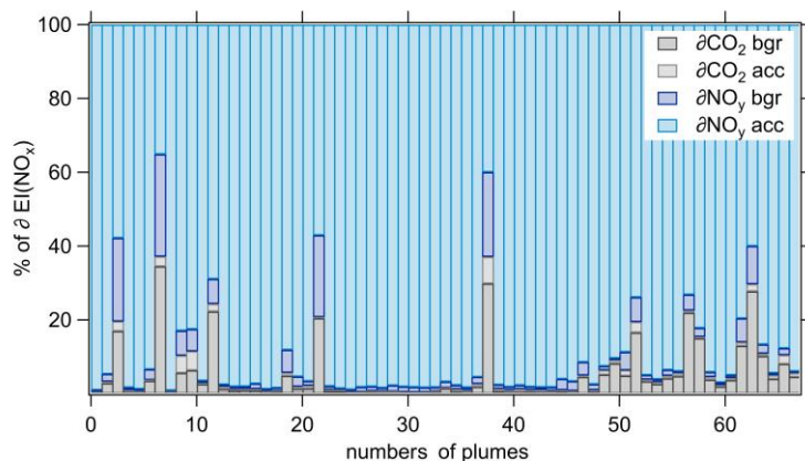
hence, \text{NO}_y is taken as the main focus for this determination. If prior and after the encounter the mole fractions are identical, Figure 9: Stacked relative individual uncertainties contributing to the total uncertainty \delta EI(\text{NO}_x) for in-flight plume encounters.
