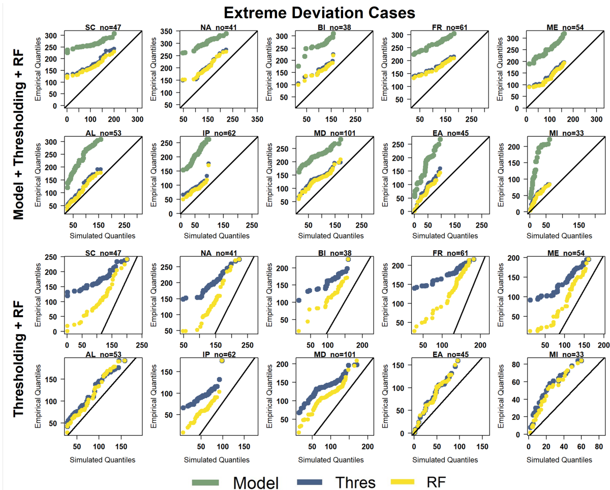
Figure 7. QQ Plots Comparing the Number of Rainy Days in Extreme Deviation Cases: Simulated values from the first model (redgreen) and their respective corrected values derived from both the thresholding method (blue) and the RF method (orangeyellow) are depicted. The first set of QQ plots displays outcomes for the 10 sub-areas, encompassing the model values. The second set illustrates the identical outcomes, specifically focusing on the BC methods.
