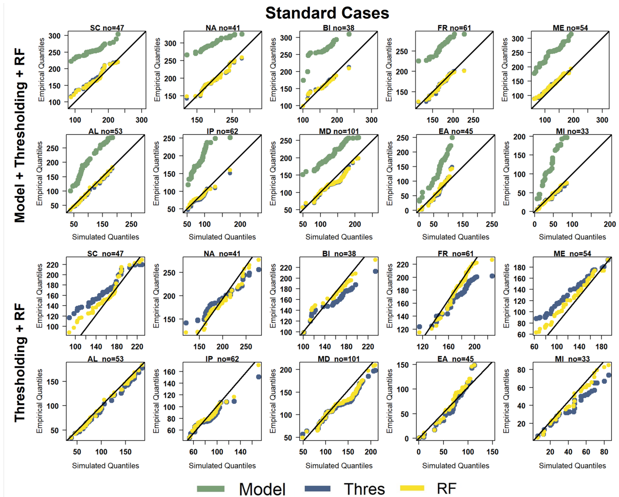
Figure 6. Q-Q Plots Comparing the number of rainy days (per year) for the default evaluation period (2001-2005): Simulated values from the first model (redgreen) and their respective corrected values derived from both the thresholding method (blue) and the RF method (orangeyellow) are depicted. The first set of Q-Q plots displays outcomes for the 10 sub-areas, encompassing the model values. The second set illustrates the identical outcomes, specifically focusing on the BC methods.
