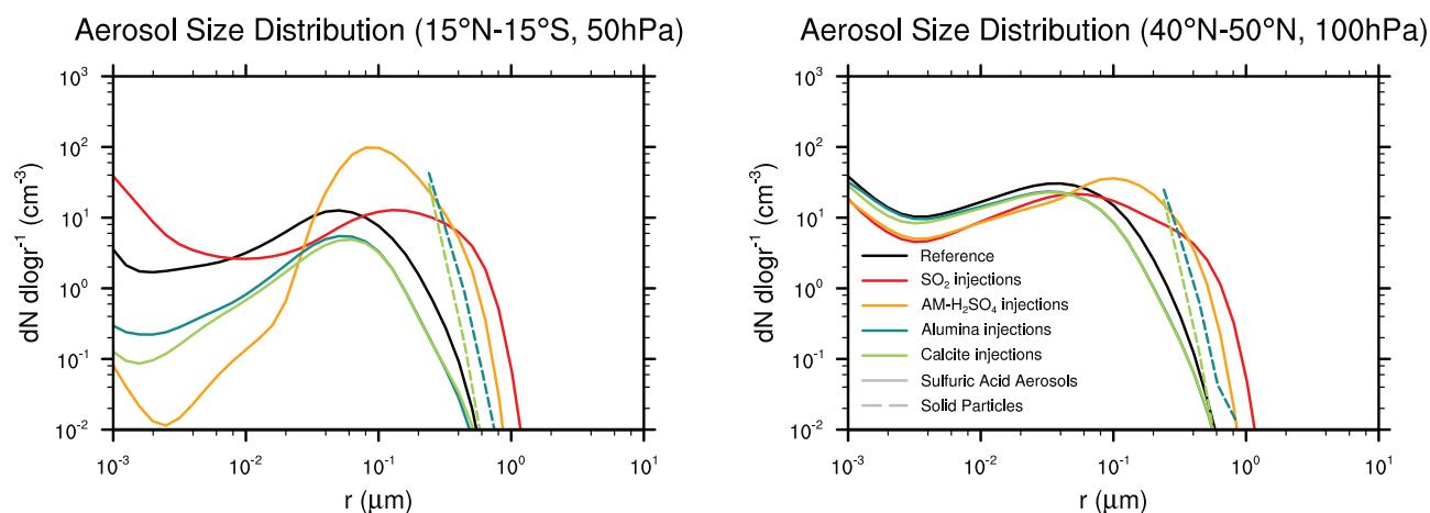
Figure S7. The resulting aerosol size distribution averaged between 15°N and 15°S at 50 hPa altitude (a) and between 40°N and 50°N at 100 hPa altitude (b). Solid lines show the sulfuric acid aerosol size distribution and dashed lines the solid particle size distributions for the 5 Mt/yr injection scenarios as well as the reference simulation (black).
