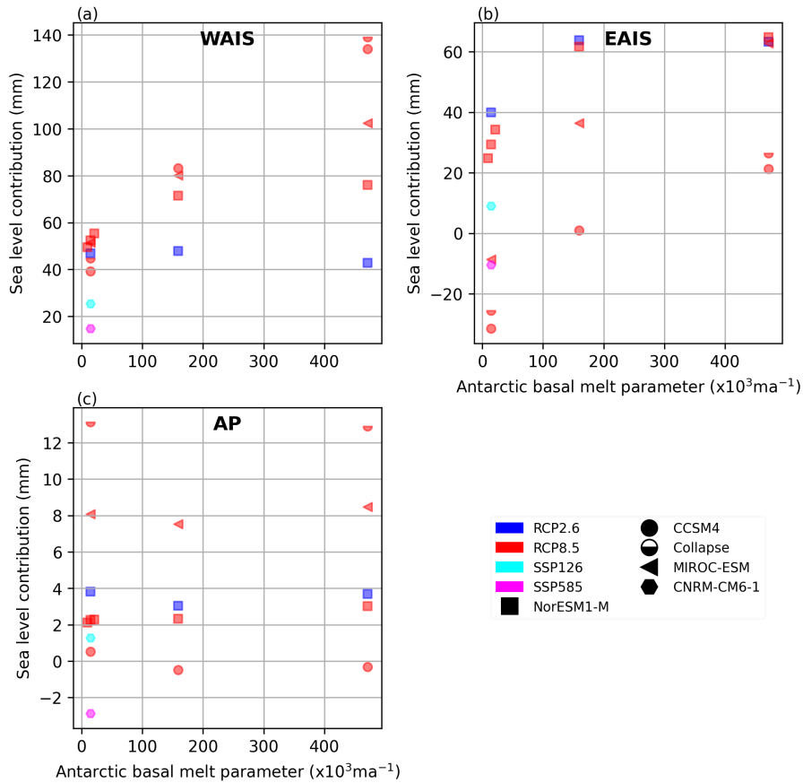
Figure 10. Sea level contribution from 2015 to 2100 for all simulations as a function of basal melt sensitivity ( \gamma_0 ), shown for West Antarctic (WAIS) (a) East Antarctic (EAIS) (b) , and Peninsula (AP) (c) ice sheets.
