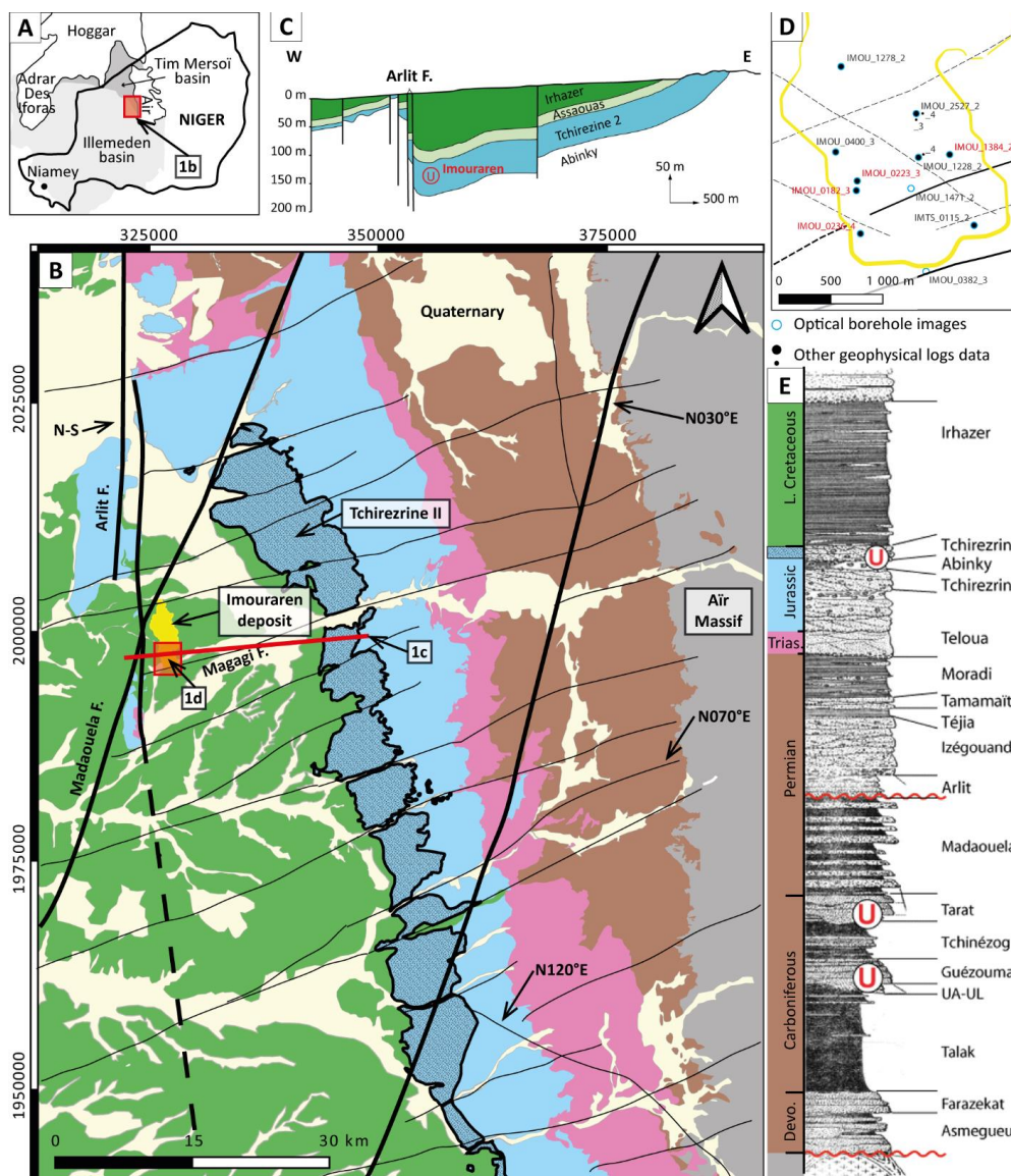
Figure 1: (A) Location map of the Tim Mersoï basin in North-Niger. (B) Geological map of the study area showing the location of the Tchirezrine II outcrop and the Imouraren site. (C) Cross-section between Arlit fault and Tchirezrine II outcrop (Orano internal report). (D) Location of the studied wells within the Imouraren site, red wells are ones from Figures 7d, 8d and 10c. (E) Lithostratigraphy modified from Gerbeaud (2006).
