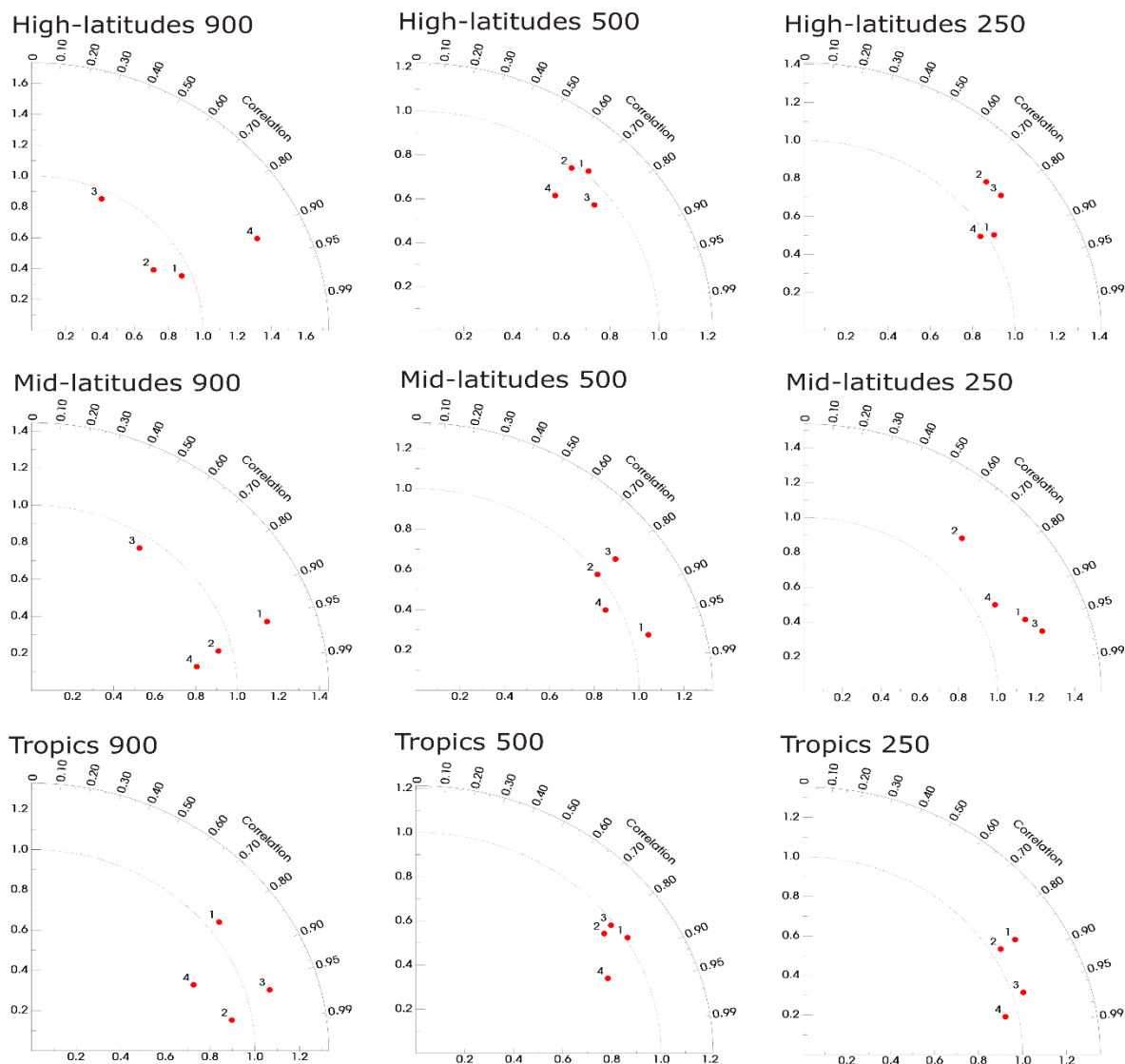
890 Fig. 2: Taylor diagram of comparisons between modelled monthly mean ozone climatology (2000-2018) and ozone sonde climatology (1995-2010) data from Tilmes et al. 2012 in the high Tropics (bottom), mid-latitudes (middle), and high latitudes (top) for three different altitude levels (900 hPa, 500 hPa and 250 hPa) in the troposphere. The x-axis shows the relative ozone normalized bias of the simulations compared to the observations, whereas the radial in the y-axis describes the correlation coefficient of seasonal averaged ozone values between simulated and observed values. Numbers indicate 895 different regions as difference in previous studies 26,40 . Bottom panels: 1-NH Subtropics; 2-W-Pacific/E-India Ocean; 3- equat. America; 4-Atlantic/Africa; Middle panels: 1-Western Europe; 2-Eastern US; 3-Japan; 4-SH Mid Latitudes; Top panels: 1-NH Polar West; 2-NH Polar East; 3-Canada; 4-SH Polar.
