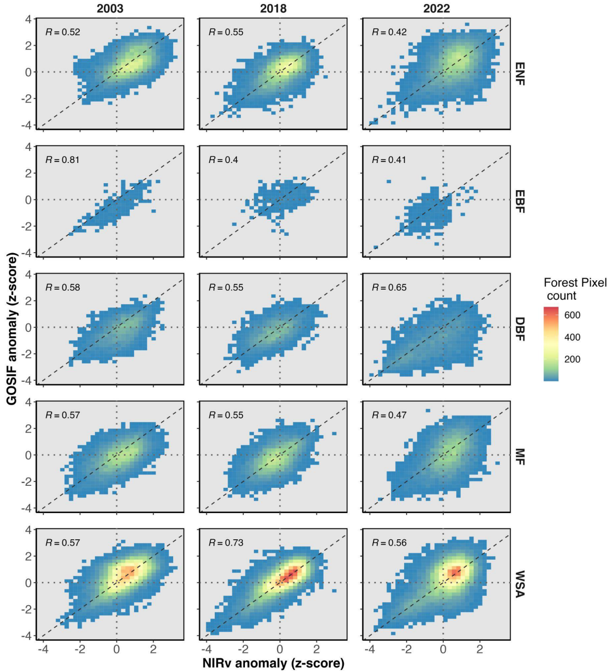
Supplementary Figure 1 Relationship between SIF and NIRv anomalies during 2003, 2018, and 2022 for different forest types.
