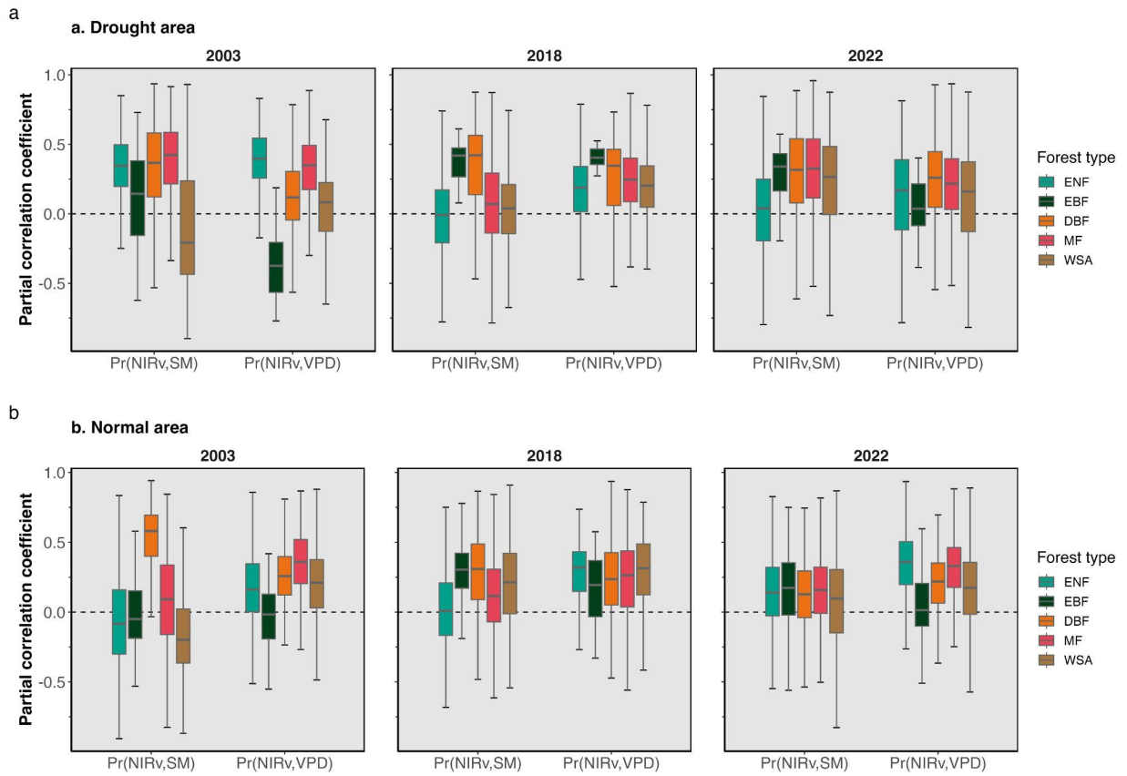
Supplementary Figure 2 Temporal partial correlation coefficient of NIRv with SM and VPD during summer for detected (a) drought areas and (b) normal areas.
