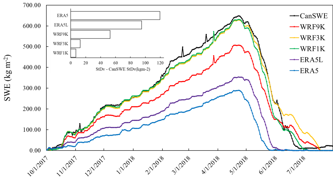
275 Figure 2. Temporal variation of SWE, from CanSWE data, WRF model resolutions, ERA5L and ERA5 over the SSRB region. The SWE data are aggregated for all stations inside the innermost domain. The spikes in the graph correspond to snowfall events, indicating the accumulation and subsequent melting of snow. The difference between CanSWE StDv and the StDv of each dataset is shown in the upper left.
