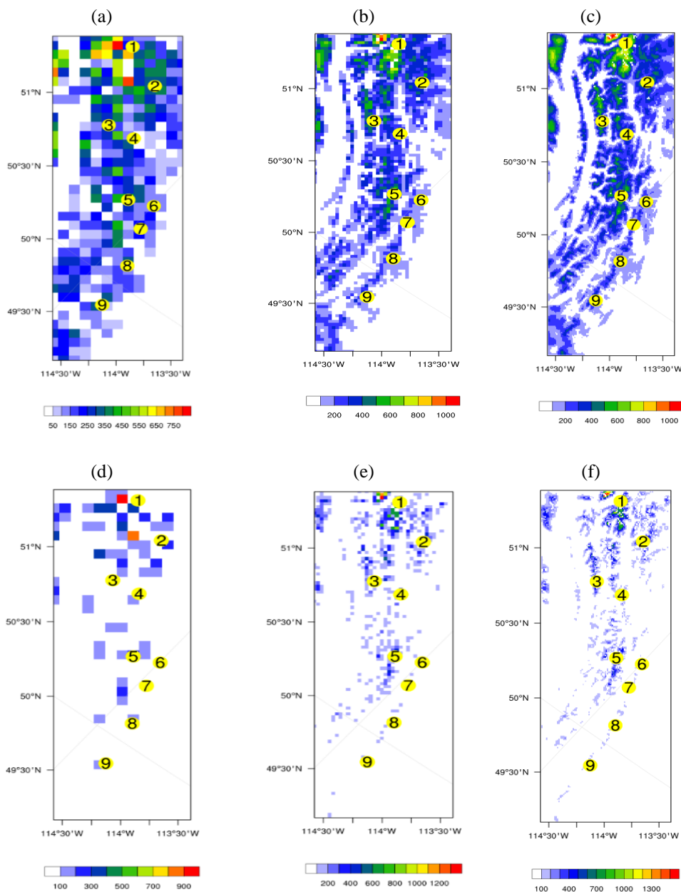
335 Figure 6. Simulated mean SWE ( \text{kg/m}^2 ) during the accumulation (1st October 2017- 22nd April 2018) and melting (23rd April 2018 to 1st October 2018) period for WRF9K (a,d), WRF3K(b,e) and WRF1K (c,f) over the inner model domain.
