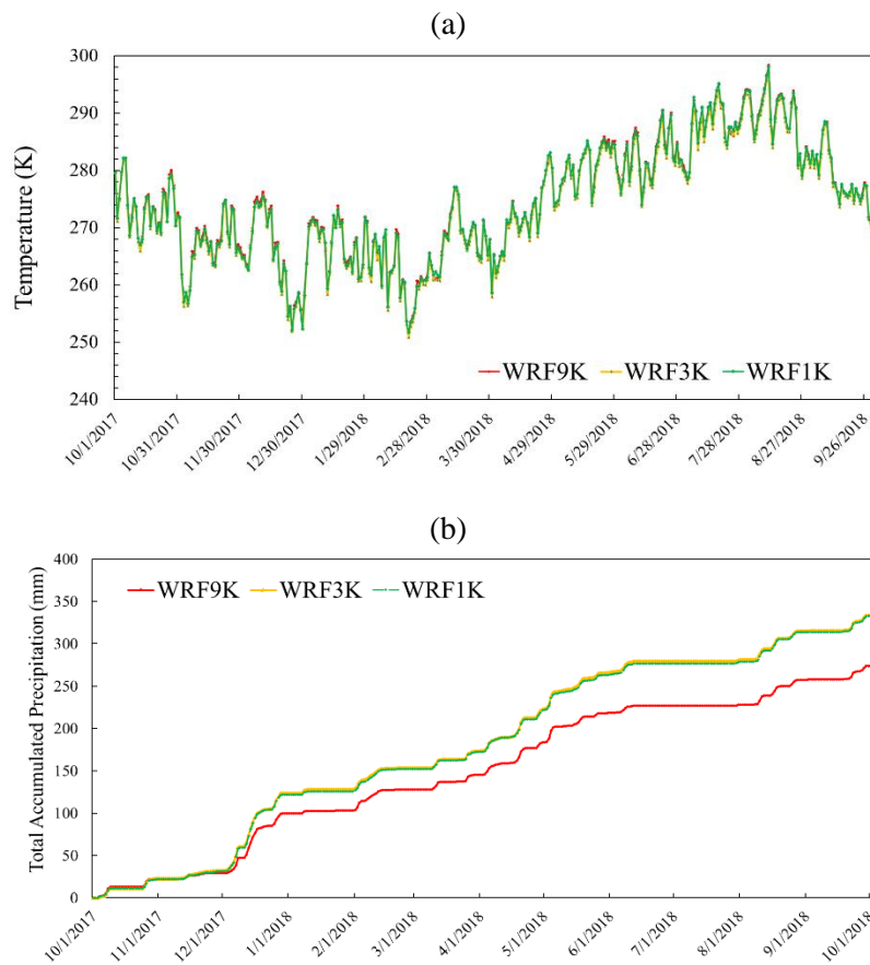
280 Figure 3. Temporal variation of 2m temperature (a) and precipitation (b) from the three WRF model resolutions over the SSRB region for the innermost domain.
