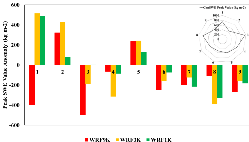
370 Figure 8. The anomalies in the value WRF maximum SWE estimation for each station during 1 st October 2017-2018. The anomaly shows how much the value of SWE is estimated more/less at each resolution (1 to 9). The value of maximum SWE for CanSWE at each station is shown in the upper right.
