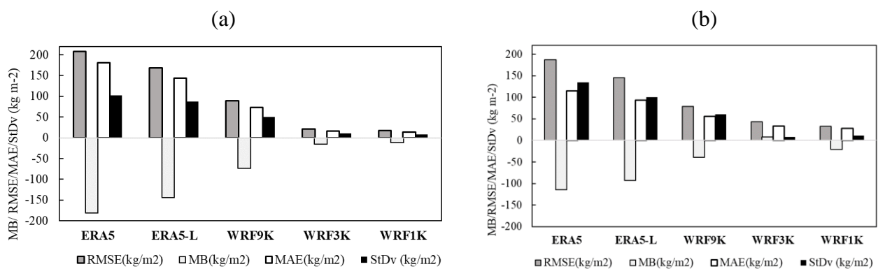
295 Figure 4. SWE evaluation during (a) accumulation period (1st October 2017- 22nd April 2018) and (b) melting period (23rd April 2018 to 1st October 2018) over the inner WRF model domain using RMSE, MB, MAE and StDv .
