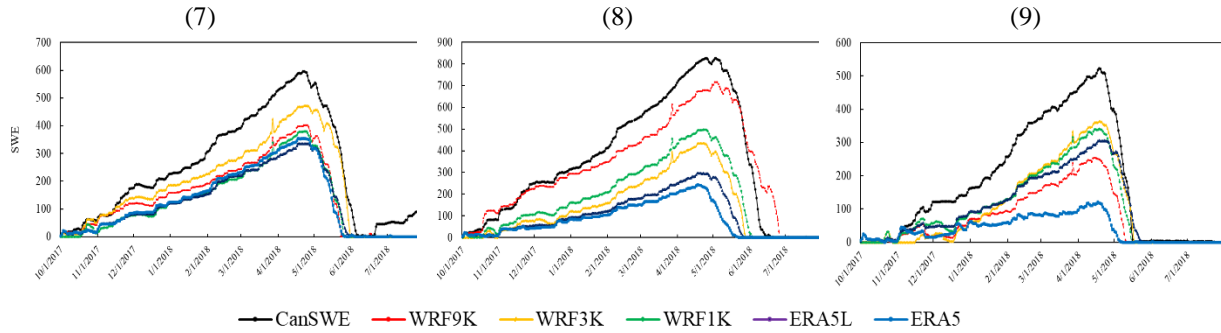
Figure 5. Estimation of SWE using WRF comparing to the CanSWE data for station 1 to 9.
