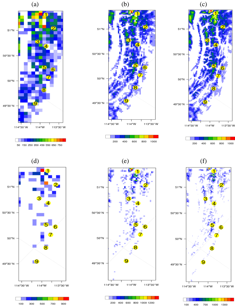
Figure 6. Simulated mean SWE ( \text{kg}/\text{m}^2 ) during the accumulation (1st October 2017- 22nd April 2018) and melting (23rd April 2018 to 1st October 2018) period for WRF9K (a,d), WRF3K(b,e) and WRF1K (c,f) over the inner model domain.
