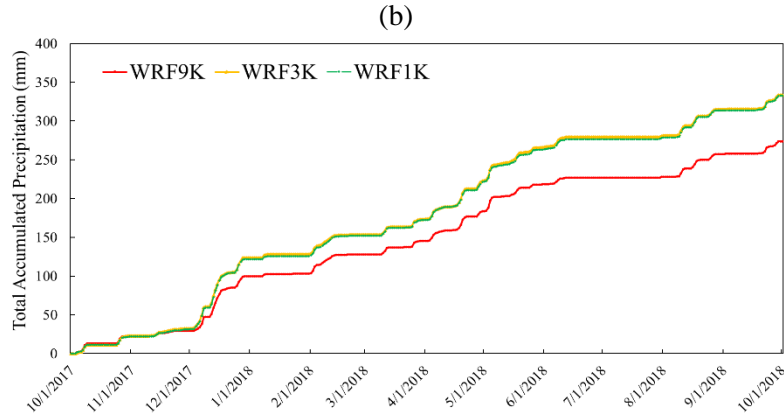
Figure 3. Temporal variation of 2m temperature (a) and precipitation (b) from the three WRF model resolutions over the SSRB region for the innermost domain.
